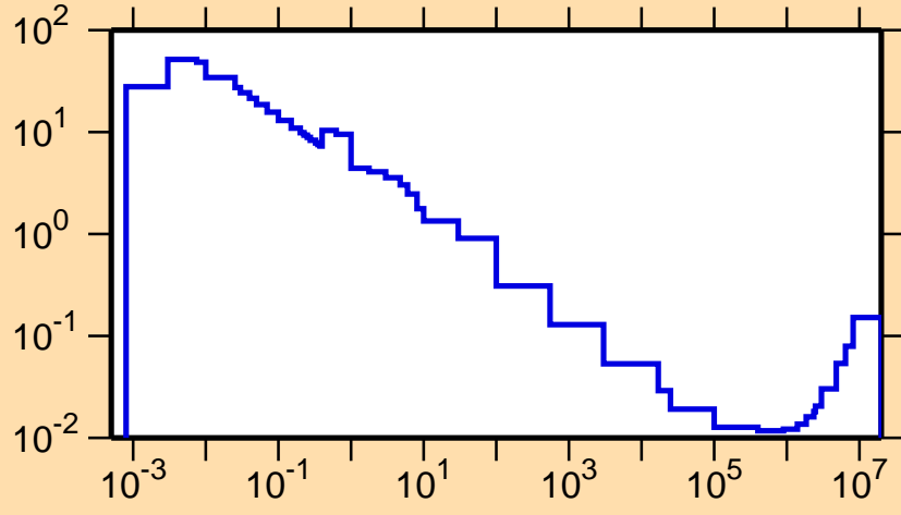
\sigma vs. E for ^{172}\text{Ir}(n,\alpha)
