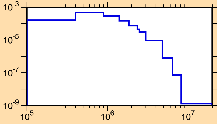
\sigma vs. E for ^{172}\text{Ir}(n,n_1)
