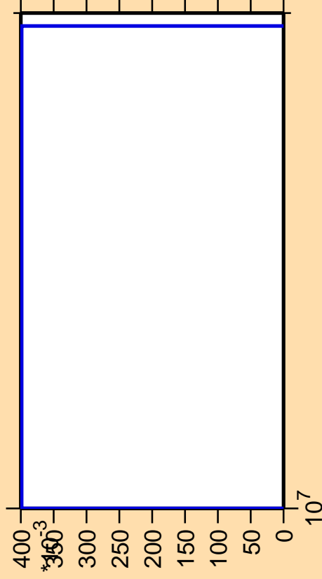
\Delta\sigma/\sigma vs. E for ^{179}\text{Ir} (mt 34)
