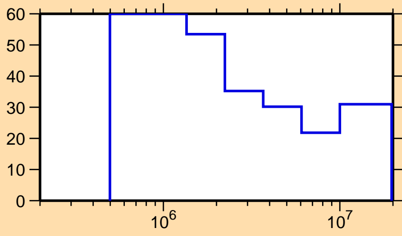
\Delta\sigma/\sigma vs. E for ^{179}\text{Ir}(n,n\text{cont.})
