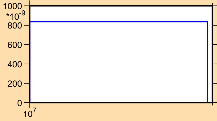
\sigma vs. E for ^{179}\text{Ir}(n,3n)
