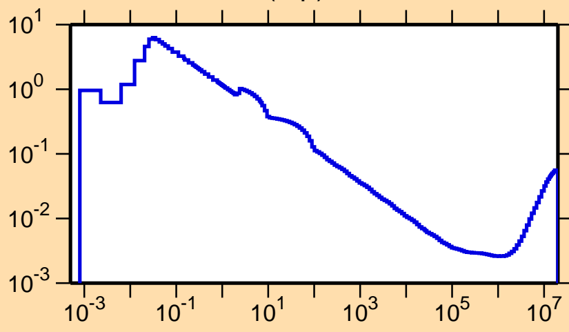
\sigma vs. E for ^{182}\text{Ir}(n,p)
