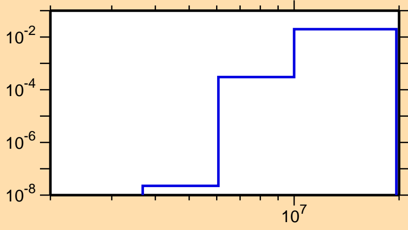
\sigma vs. E for ^{182}\text{Ir}(n,np)
