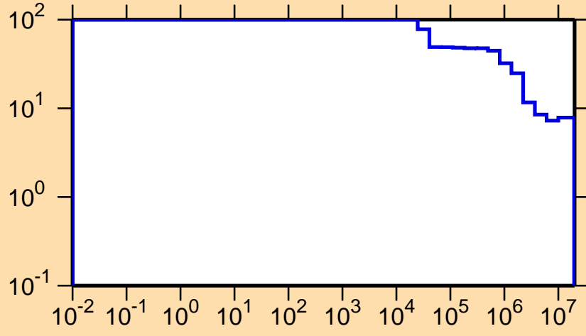
\Delta\sigma/\sigma vs. E for ^{182}\text{Ir}(n,\text{nonel.})
