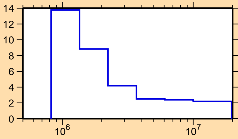
\Delta\sigma/\sigma vs. E for ^{188}\text{Ir}(n, n_{\text{nonel}})
