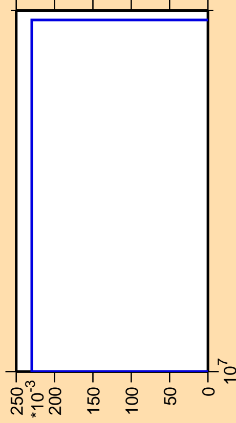
\Delta\sigma/\sigma vs. E for ^{188}\text{Ir} (mt 45)
