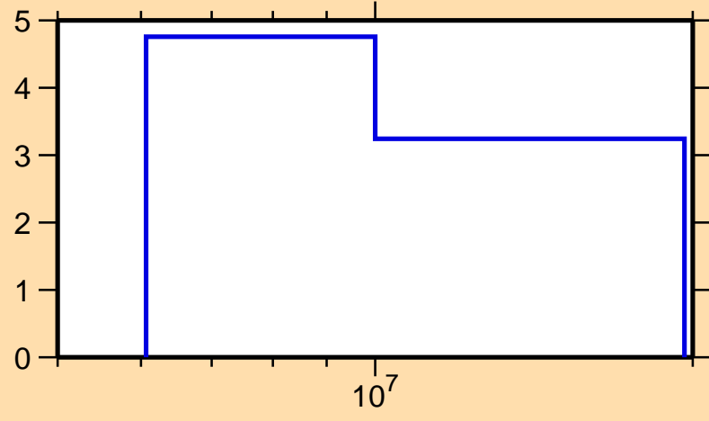
\Delta\sigma/\sigma vs. E for ^{188}\text{Ir}(n,\text{el.})
