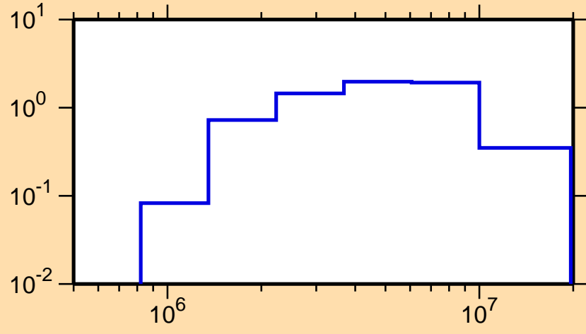
\sigma vs. E for ^{188}\text{Ir}(n,n\text{cont.})
