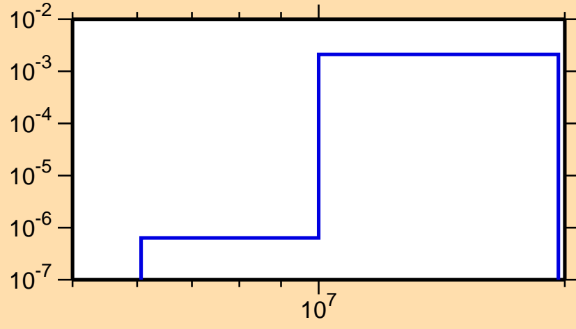
\sigma vs. E for ^{188}\text{Ir}(n,np)
