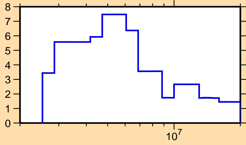
\Delta\sigma/\sigma vs. E for ^{193}\text{Ir}(n,el.)
