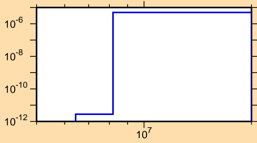
\sigma vs. E for ^{193}\text{Ir}(n,n\alpha)
