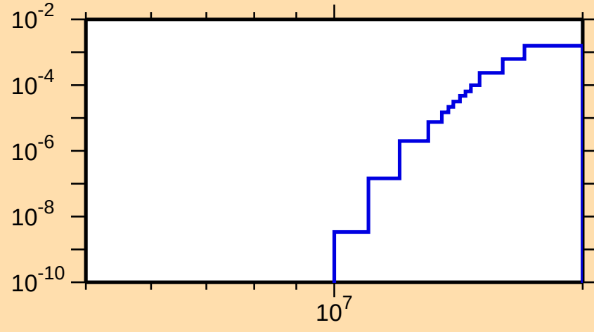
\sigma vs. E for ^{195}\text{Ir}(n,np)
