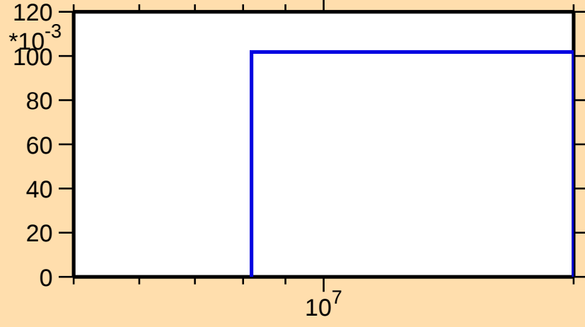
\sigma vs. E for ^{195}\text{Ir}(n,3n)
