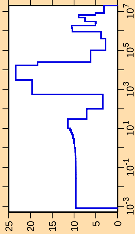
\Delta\sigma/\sigma vs. E for ^{195}\text{Ir}(n,\text{el.})
