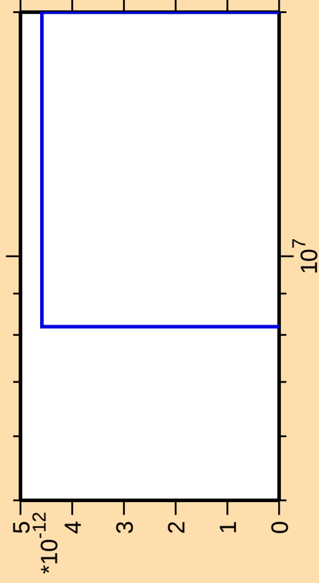
\Delta\sigma/\sigma vs. E for ^{195}\text{Ir}(\text{mt } 42)
