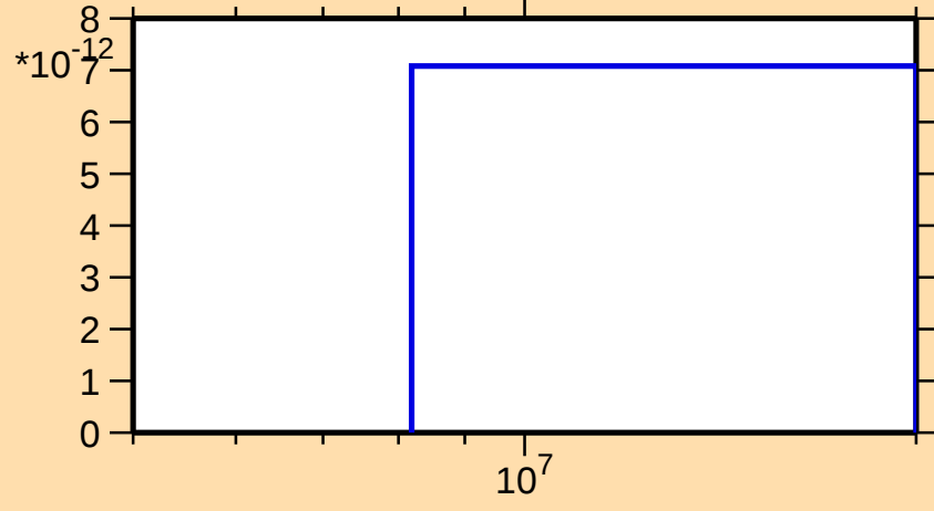
\sigma vs. E for ^{195}\text{Ir}(n,2n\alpha)
