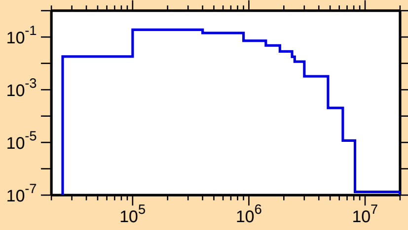
\sigma vs. E for ^{195}\text{Ir}(n,n_1)
