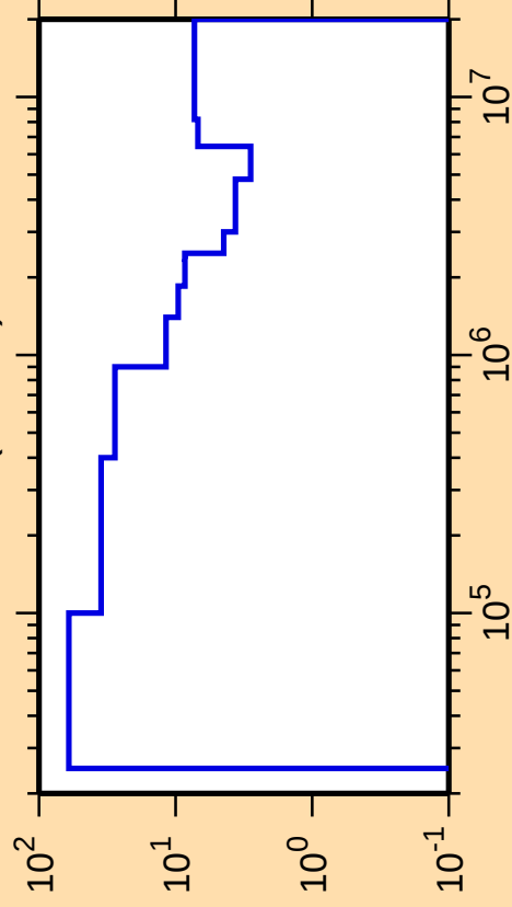
\Delta\sigma/\sigma vs. E for ^{195}\text{Ir}(\text{n,inel.})
