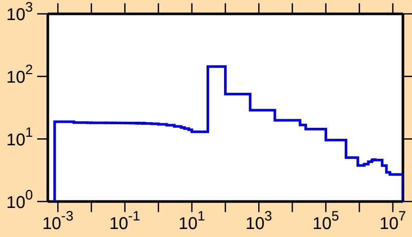
\sigma vs. E for ^{195}\text{Ir}(n,\text{el.})
