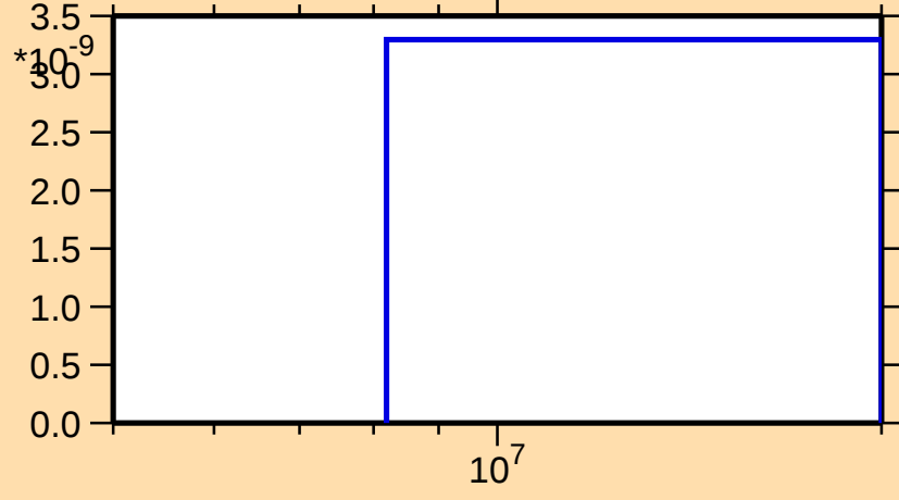
\sigma vs. E for ^{195}\text{Ir}(n,\text{nt})
