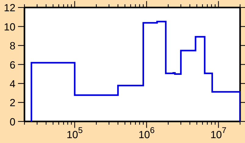
\Delta\sigma/\sigma vs. E for ^{195}\text{Ir}(\text{n,el.})
