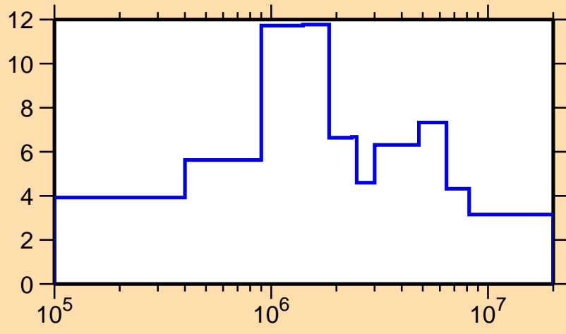
\Delta\sigma/\sigma vs. E for ^{196}\text{Ir}(n, el.)
