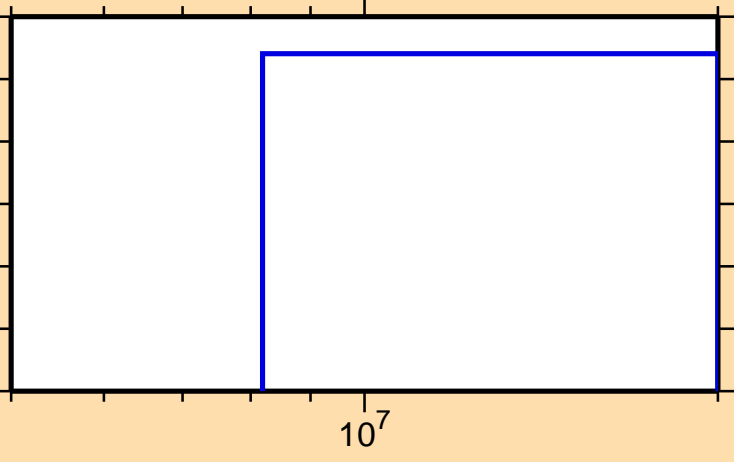
\sigma vs. E for ^{196}\text{Ir}(n,2np)
