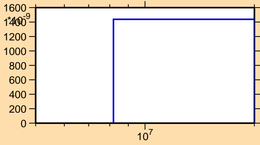
\sigma vs. E for ^{196}\text{Ir}(n,n\alpha)
