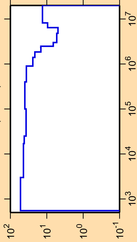
\Delta\sigma/\sigma vs. E for ^{197}\text{Ir}(n,\text{inel.})
