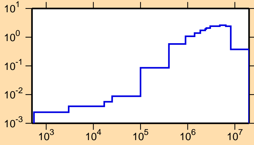
\sigma vs. E for ^{197}\text{Ir}(n,\text{inel.})
