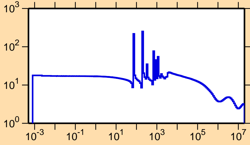
\sigma vs. E for ^{199}\text{Ir}(n,\text{el.})
