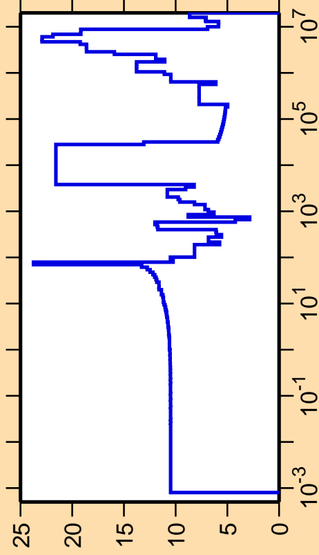
\Delta\sigma/\sigma vs. E for ^{199}\text{Ir}(n,\text{el.})
