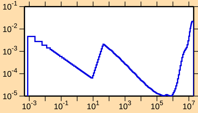
\sigma vs. E for ^{81}\text{Kr}(n,\alpha)
