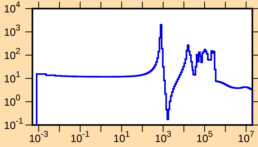
\sigma vs. E for ^{90}\text{Kr}(n,\text{tot.})
