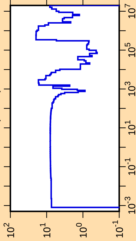
\Delta\sigma/\sigma vs. E for ^{90}\text{Kr}(n,\text{tot.})
