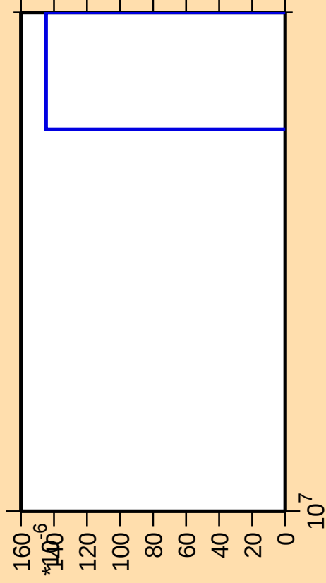
\Delta\sigma/\sigma vs. E for ^{90}\text{Kr}(n,2np)
