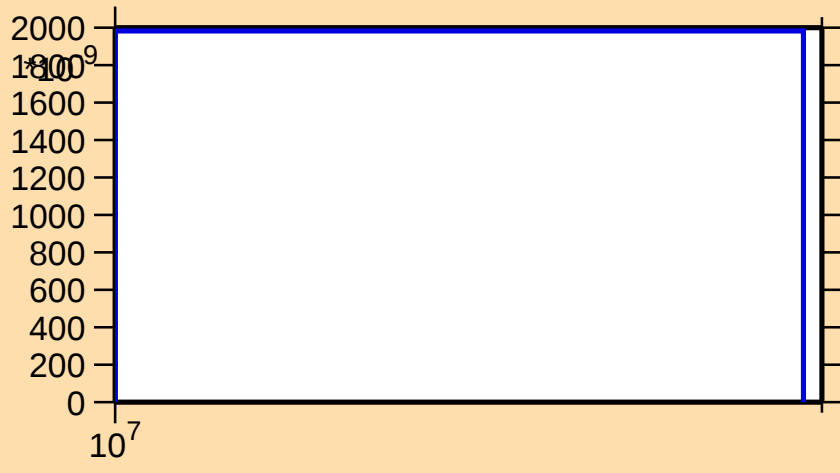
\sigma vs. E for ^{90}\text{Kr}(n,t)
