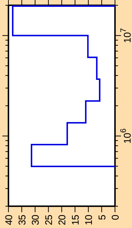
\Delta\sigma/\sigma vs. E for ^{90}\text{Kr}(n,\text{inel.})
