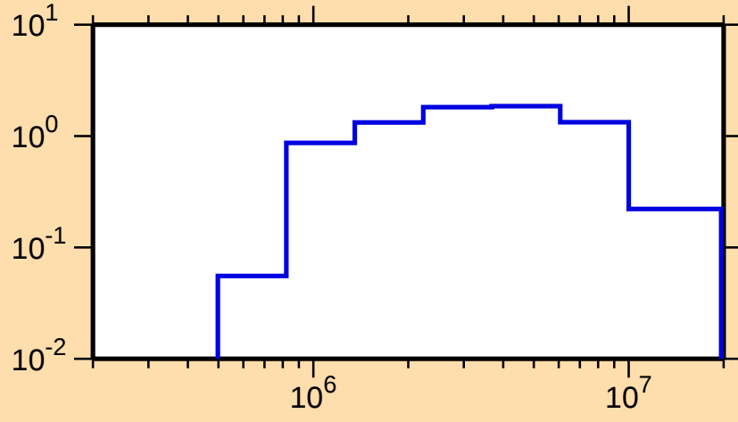
\sigma vs. E for ^{90}\text{Kr}(n,\text{inel.})
