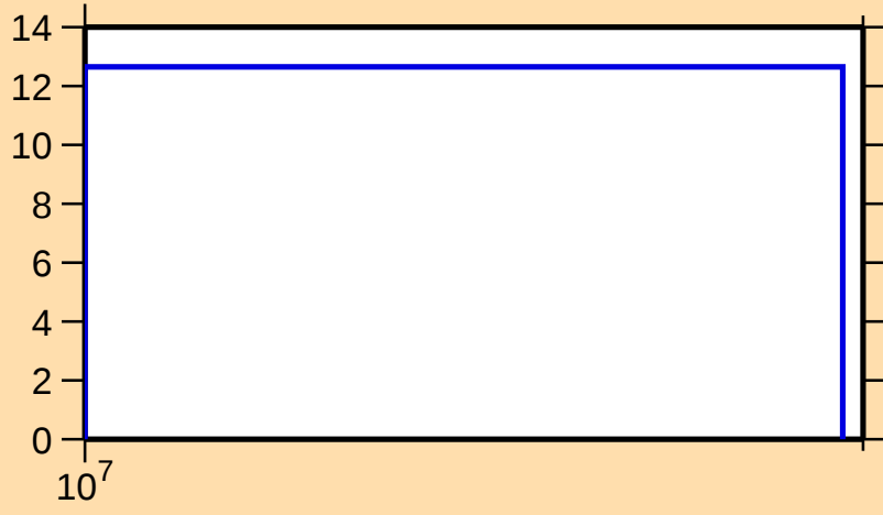
\Delta\sigma/\sigma vs. E for ^{90}\text{Kr}(n,2n)
