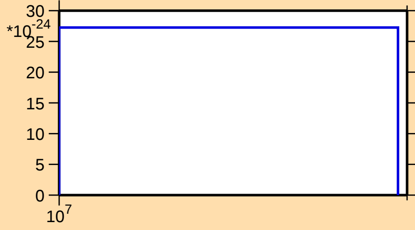
\sigma vs. E for ^{90}\text{Kr}(n,\text{He}3)
