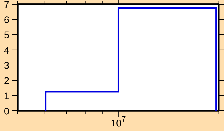
\Delta\sigma/\sigma vs. E for ^{90}\text{Kr}(n,\text{tot.})
