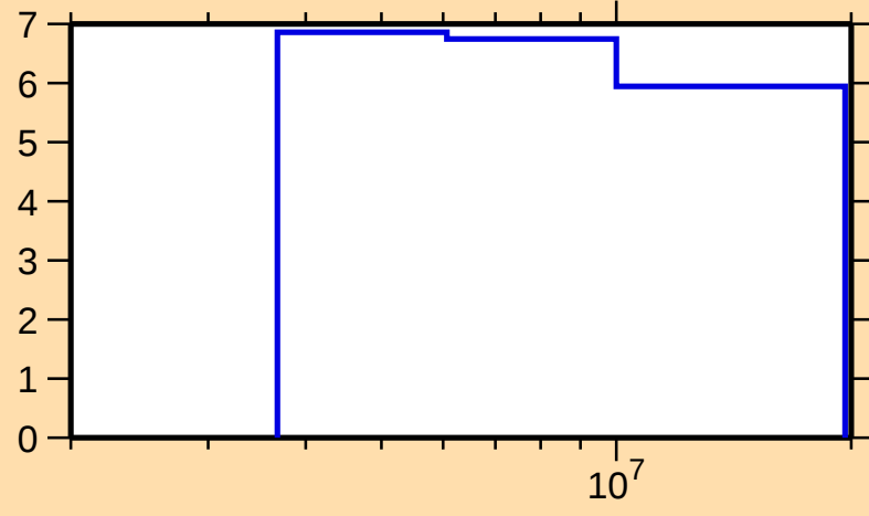
\Delta\sigma/\sigma vs. E for ^{90}\text{Kr}(\text{n},\text{nonel.})
