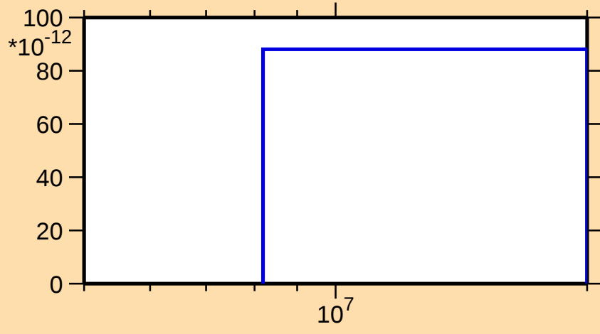
\sigma vs. E for ^{90}\text{Kr}(n,\text{nt})
