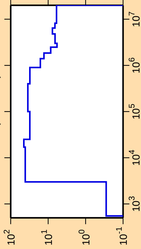
\Delta\sigma/\sigma vs. E for ^{90}\text{Kr}(n,\text{nonel.})
