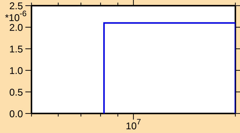
\sigma vs. E for ^{90}\text{Kr}(n,n\alpha)
