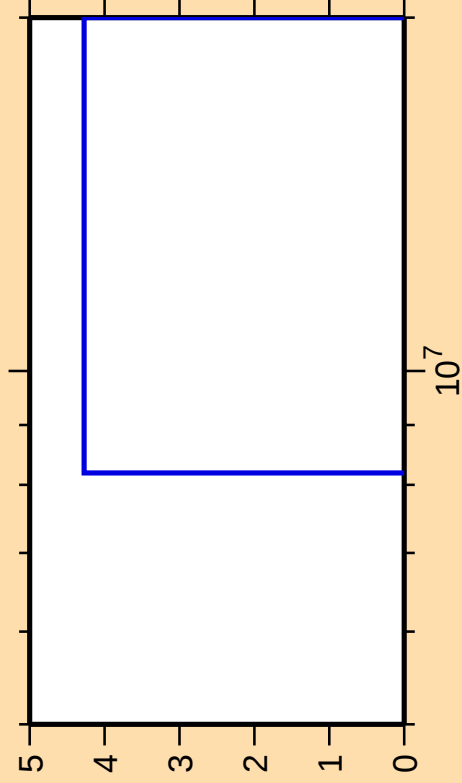
\Delta\sigma/\sigma vs. E for ^{90}\text{Kr}(n,2n\alpha)
