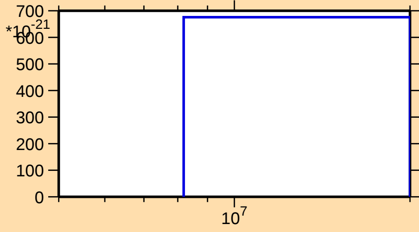
\sigma vs. E for ^{90}\text{Kr}(n,2np)
