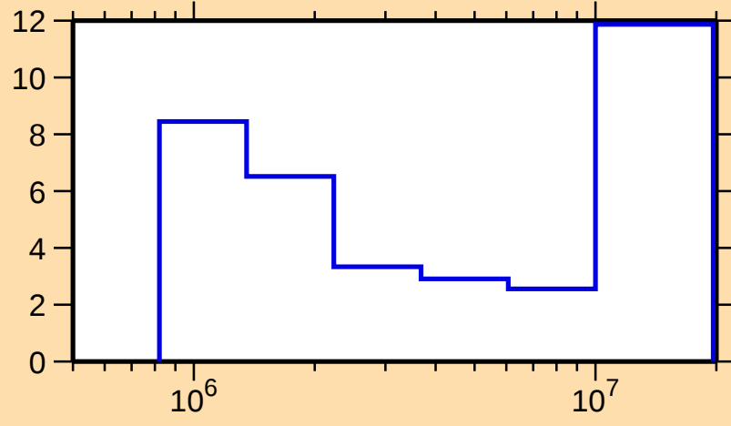
\Delta\sigma/\sigma vs. E for ^{138}\text{La}(n,n\text{cont.})
