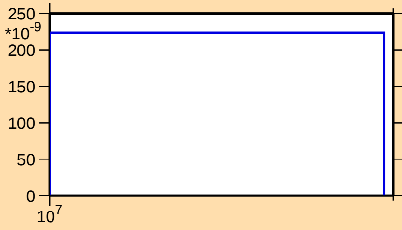
\sigma vs. E for ^{138}\text{La}(n,\text{nd})
