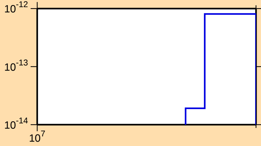
\sigma vs. E for ^{260}\text{Lw}(\text{mt } 34)
