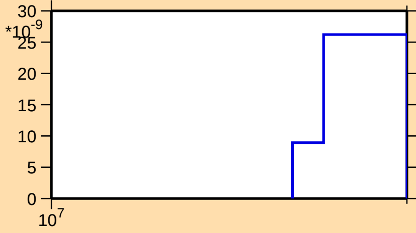
\sigma vs. E for ^{260}\text{Lw}(\text{mt117})
