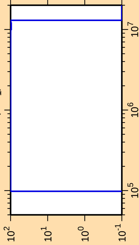
\Delta\sigma/\sigma vs. E for ^{260}\text{Lw}(n,n_1)
