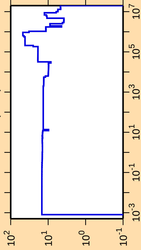
\Delta\sigma/\sigma vs. E for ^{260}\text{Lw}(n,\text{el.})
