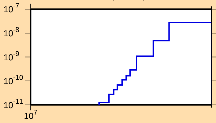
\sigma vs. E for ^{260}\text{Lw}(n,\text{He3})
