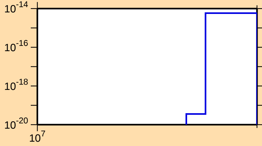
\sigma vs. E for ^{260}\text{Lw}(\text{mt 11})
