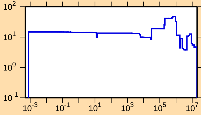
\Delta\sigma/\sigma vs. E for ^{260}\text{Lw}(n,\text{el.})
