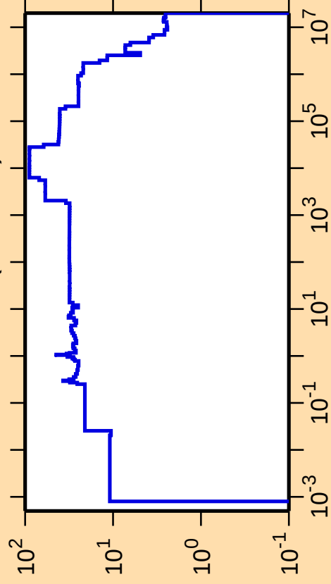
\Delta\sigma/\sigma vs. E for ^{260}\text{Lw}(n,\text{nonel.})
