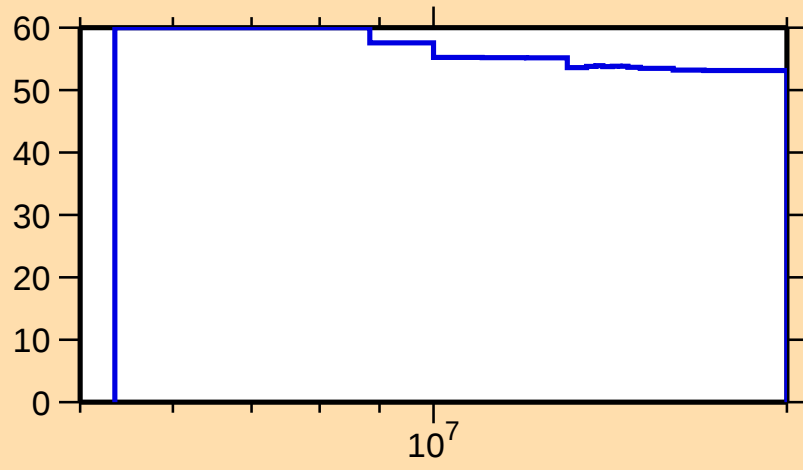
\Delta\sigma/\sigma vs. E for ^{260}\text{Lw}(n,2n)
