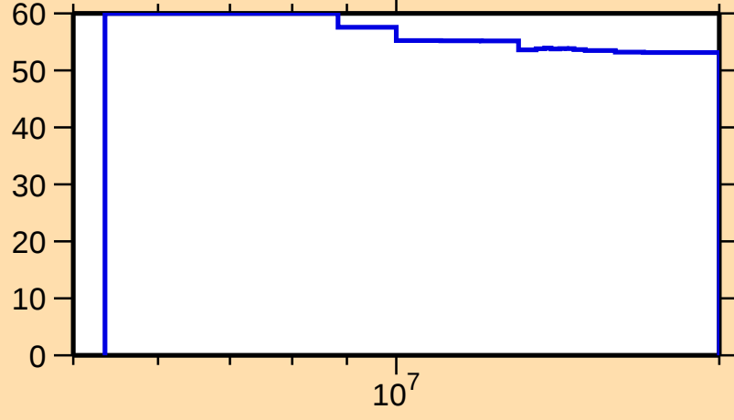
\Delta\sigma/\sigma vs. E for ^{260}\text{Lw}(n,2n)
