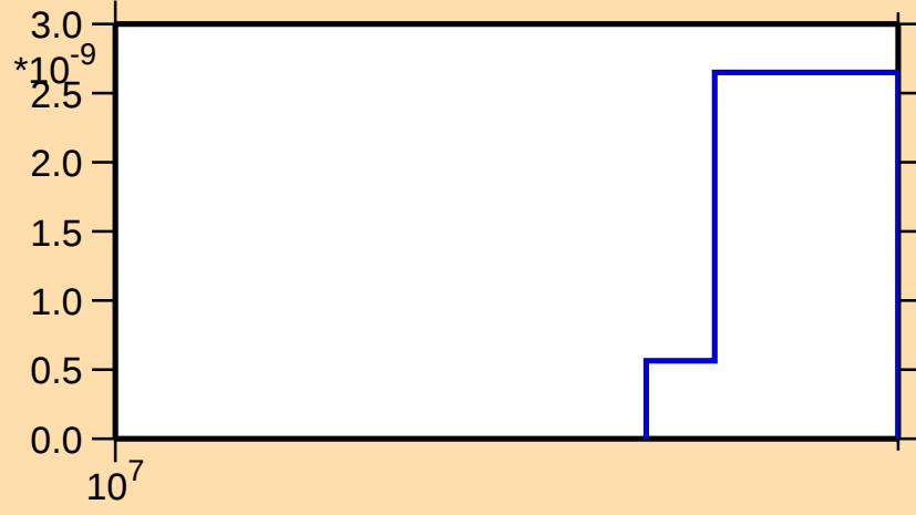
\sigma vs. E for ^{260}\text{Lw}(\text{mt 45})
