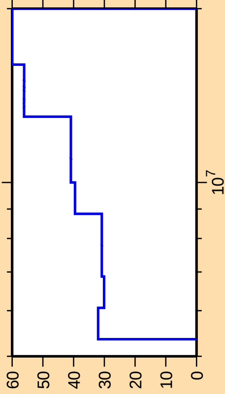
\Delta\sigma/\sigma vs. E for ^{260}\text{Lw}(n,\alpha)
