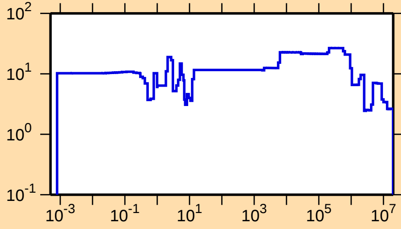
\Delta\sigma/\sigma vs. E for ^{260}\text{Lw}(n,\text{tot.})
