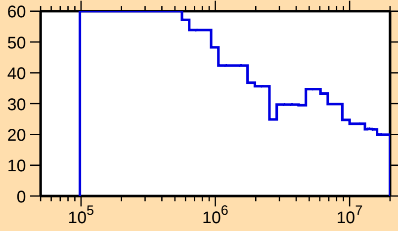
\Delta\sigma/\sigma vs. E for ^{260}\text{Lw}(n,f)
