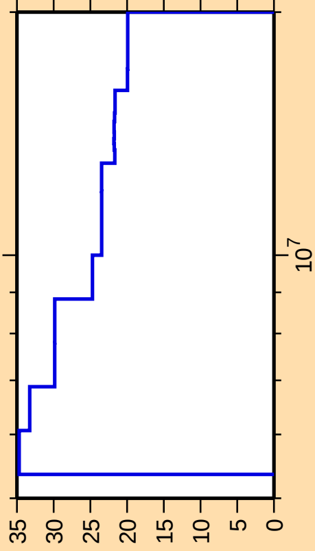
\Delta\sigma/\sigma vs. E for ^{260}\text{Lw}(n,f)
