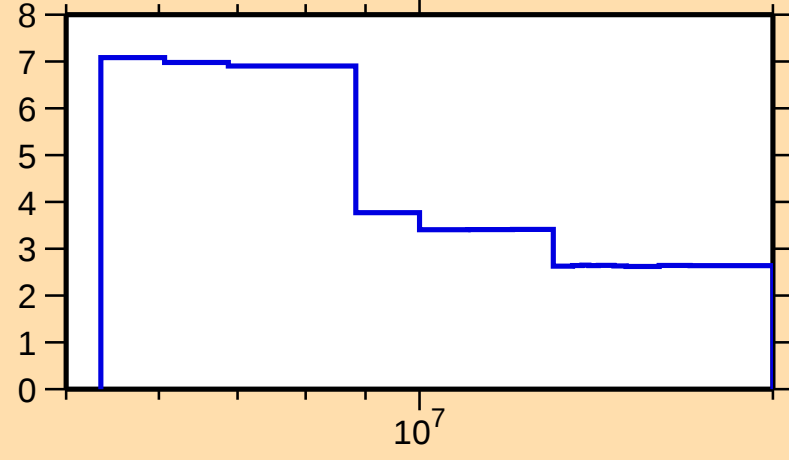
\Delta\sigma/\sigma vs. E for ^{260}\text{Lw}(n,\text{tot.})
