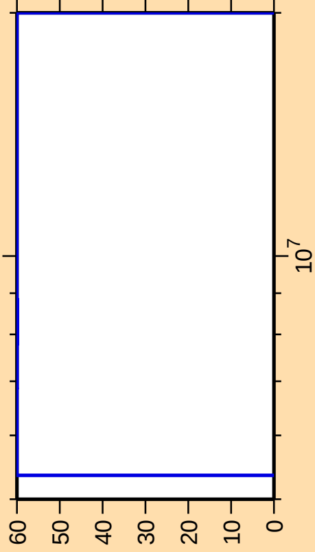
\Delta\sigma/\sigma vs. E for ^{260}\text{Lw}(n,p)
