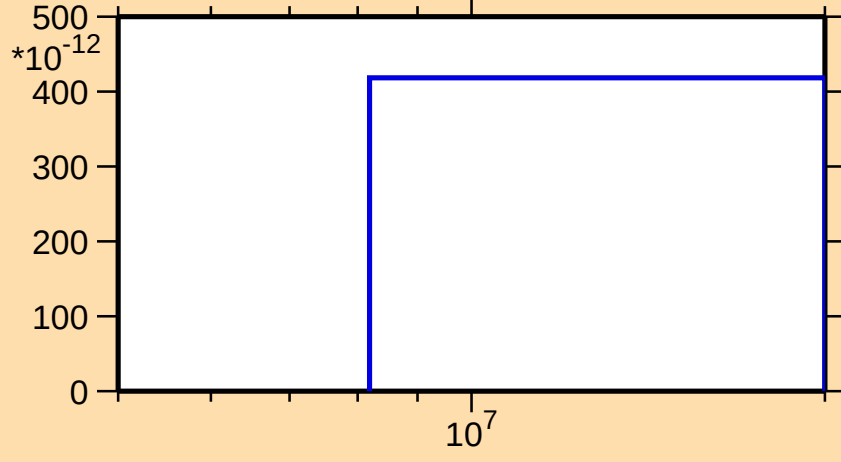
\sigma vs. E for ^{260}\text{Lw}(n,nt)
