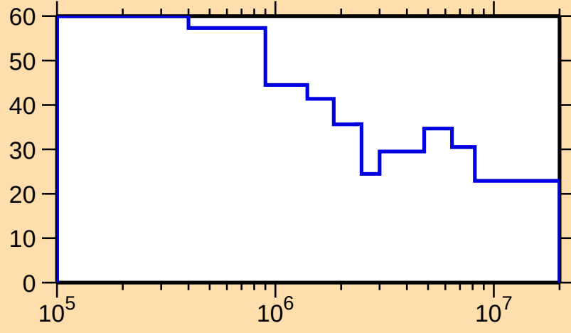
\Delta\sigma/\sigma vs. E for ^{260}\text{Lw}(n, f)
