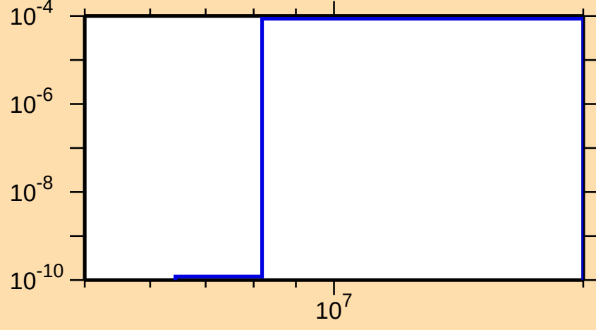
\sigma vs. E for ^{260}\text{Lw}(n,t)
