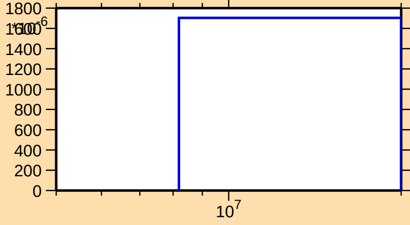
\sigma vs. E for ^{260}\text{Lw}(n,3n)
