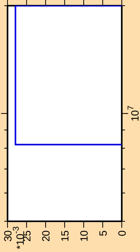
\Delta\sigma/\sigma vs. E for ^{260}\text{Lw}(\text{mt } 34)
