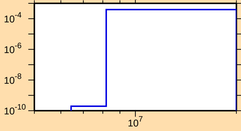
\sigma vs. E for ^{260}\text{Lw}(n,np)
