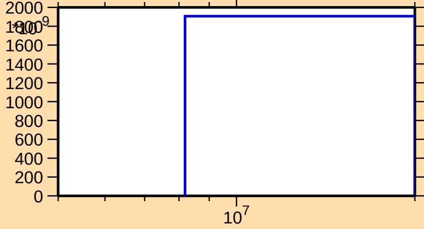
\sigma vs. E for ^{260}\text{Lw}(n,nd)
