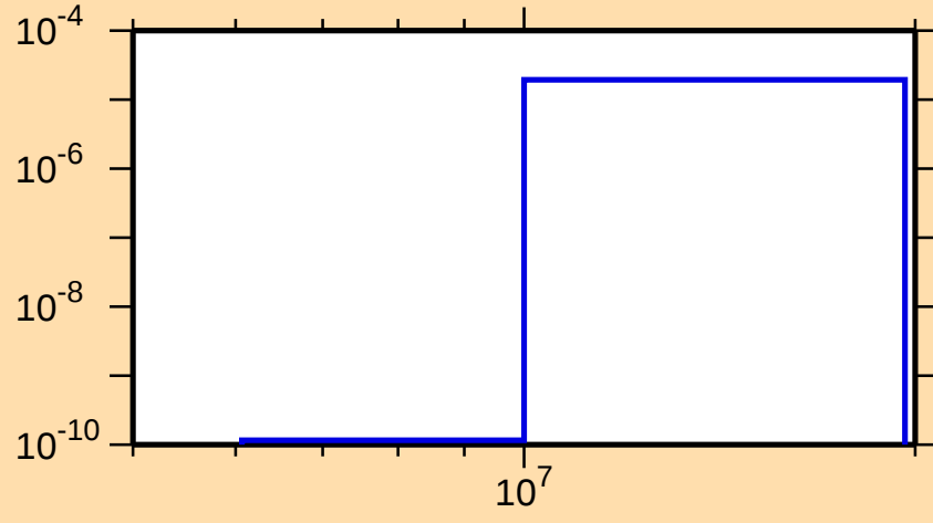
\sigma vs. E for ^{160}\text{Lu}(\text{mt } 45)
