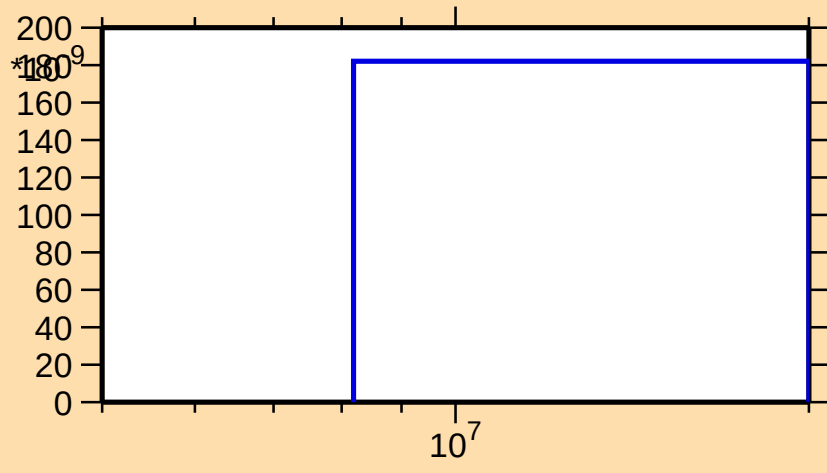
\sigma vs. E for ^{160}\text{Lu}(n,\text{pd})
