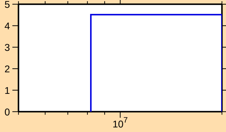
\Delta\sigma/\sigma vs. E for ^{160}\text{Lu}(n,\text{tot.})
