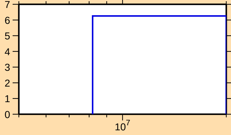
\Delta\sigma/\sigma vs. E for ^{160}\text{Lu}(n,\text{el.})
