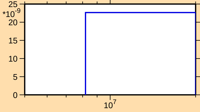
\sigma vs. E for ^{161}\text{Lu}(n,\text{pd})
