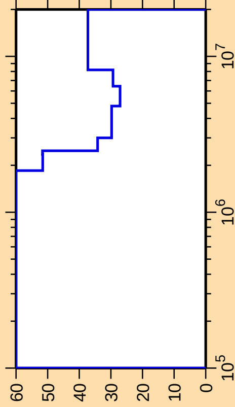
\Delta\sigma/\sigma vs. E for ^{161}\text{Lu}(n,n_{\text{cont}})
