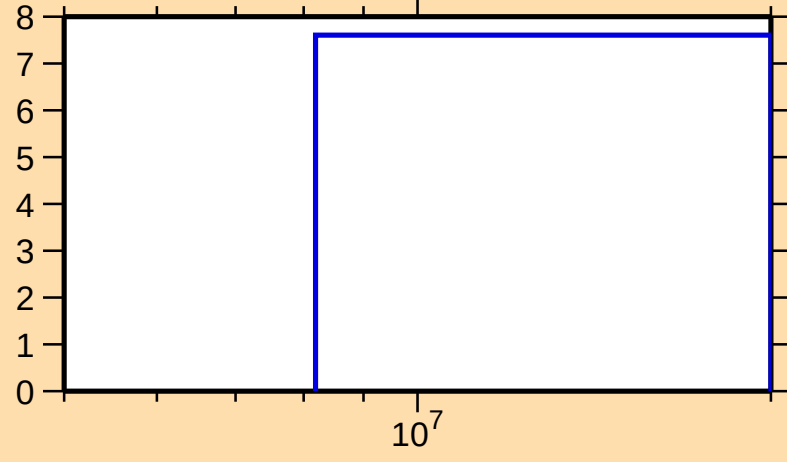
\Delta\sigma/\sigma vs. E for ^{161}\text{Lu}(n,\text{el.})
