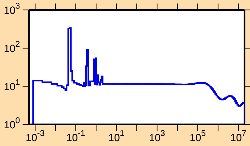
\sigma vs. E for ^{291}
