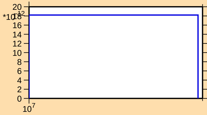
\sigma vs. E for ^{291}\text{He3} )
