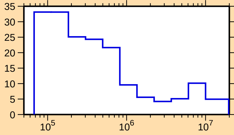
\Delta\sigma/\sigma vs. E for ^{291}
