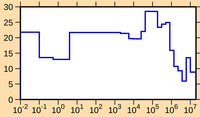
\Delta\sigma/\sigma vs. E for ^{291}
