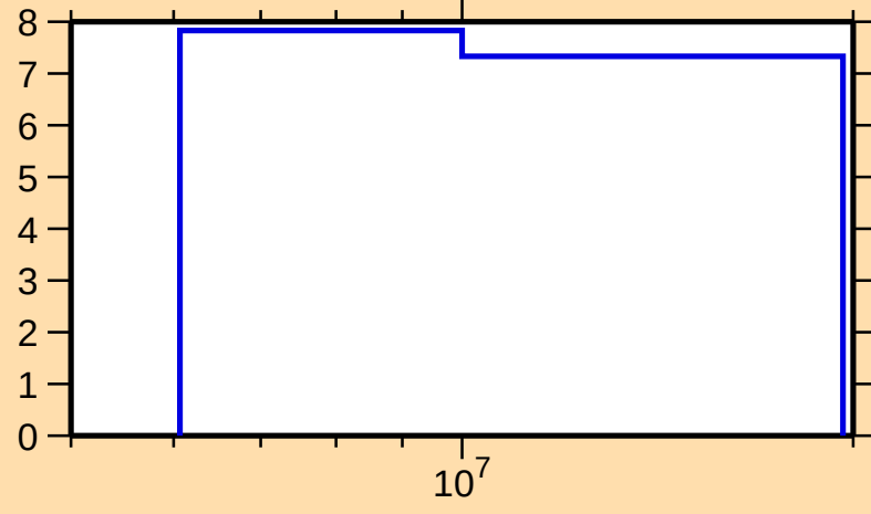
\Delta\sigma/\sigma vs. E for ^{291}
