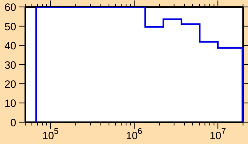
\Delta\sigma/\sigma vs. E for ^{291}_1
