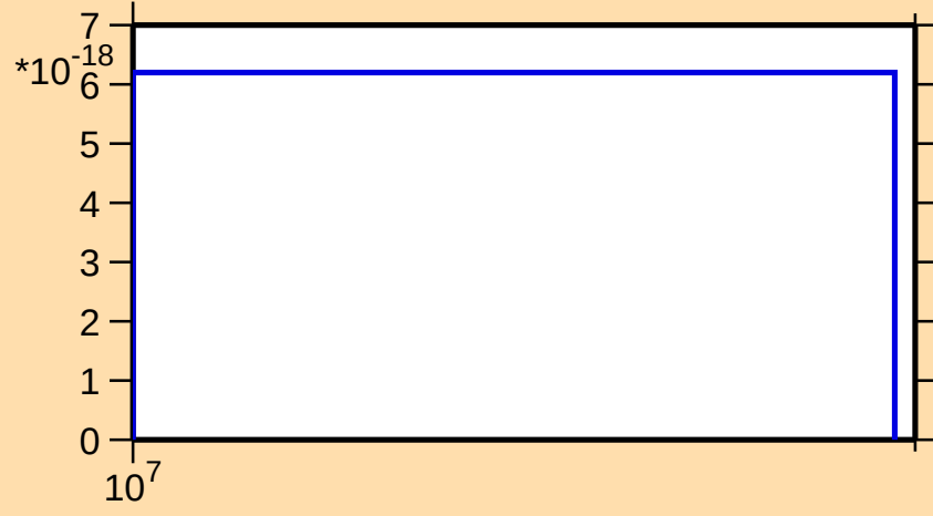
\sigma vs. E for ^{291}
