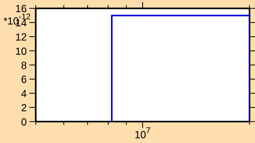
\sigma vs. E for ^{291}\text{He3}
