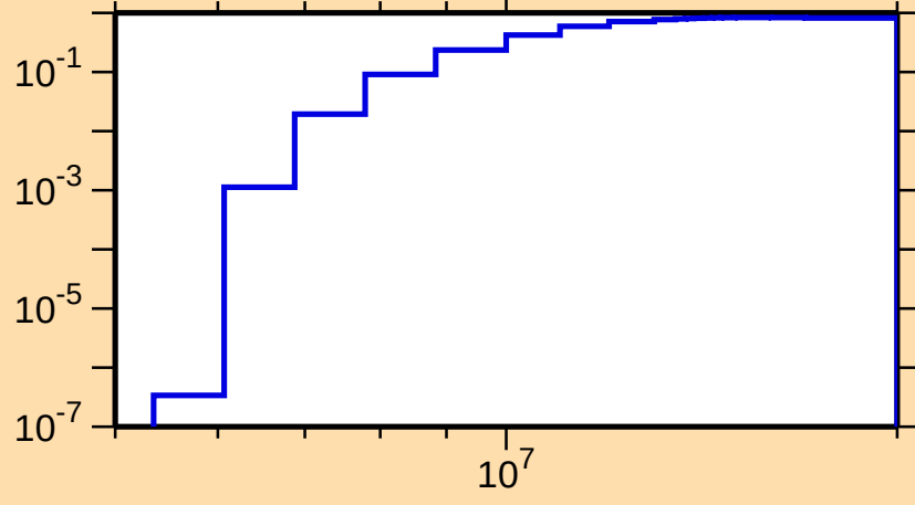
\sigma vs. E for ^{51}\text{Mn}(n,np)
