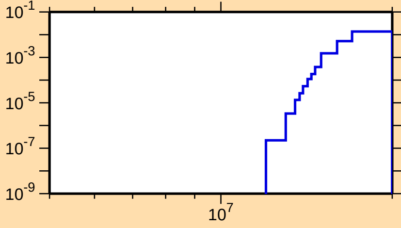
\sigma vs. E for ^{51}\text{Mn}(n,n\alpha)
