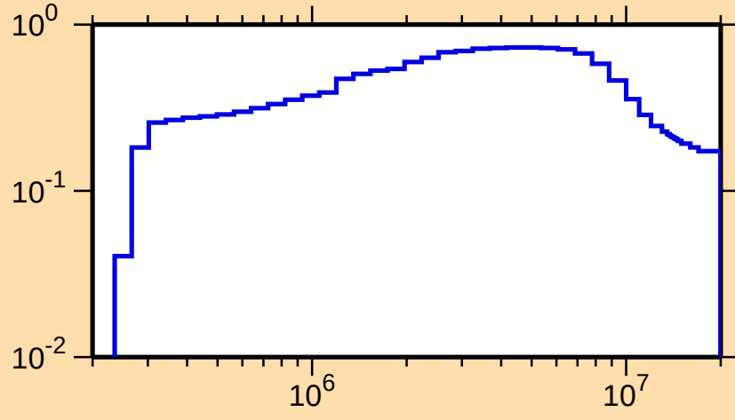
\sigma vs. E for ^{51}\text{Mn}(n,\text{inel.})
