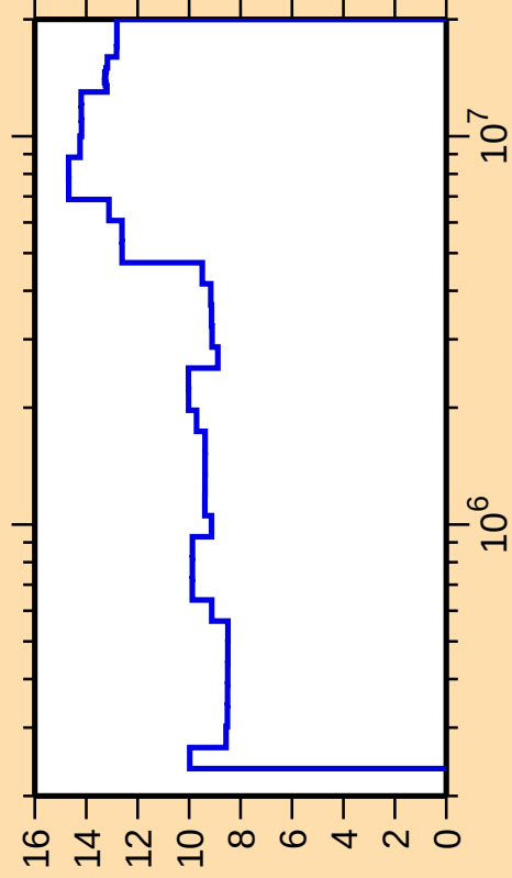
\Delta\sigma/\sigma vs. E for ^{51}\text{Mn}(n,n_1)
