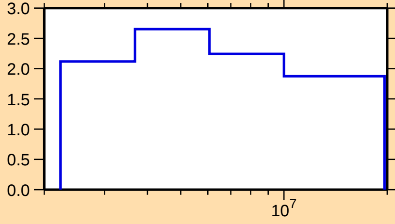
\Delta\sigma/\sigma vs. E for ^{51}\text{Mn}(n,n\text{oncl.})
