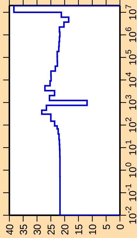
\Delta\sigma/\sigma vs. E for ^{51}\text{Mn}(n,\gamma)
