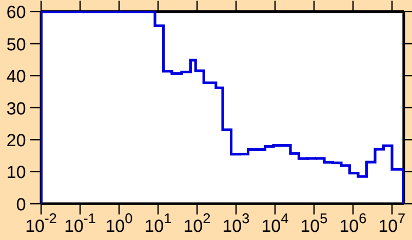
\Delta\sigma/\sigma vs. E for ^{51}\text{Mn}(n,p)
