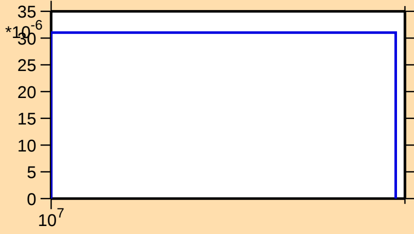
\sigma vs. E for ^{51}\text{Mn}(n,t)
