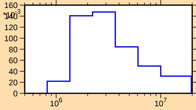
\sigma vs. E for ^{51}\text{Mn}(n,n_2)
