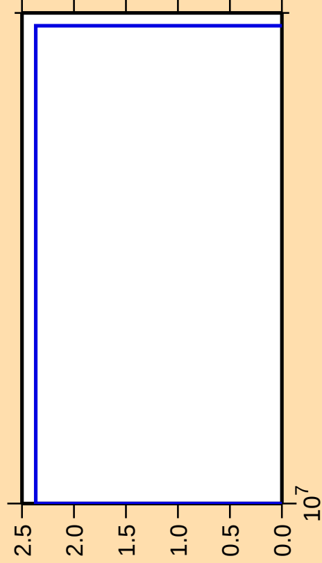
\Delta\sigma/\sigma vs. E for ^{51}\text{Mn} (mt 45)
