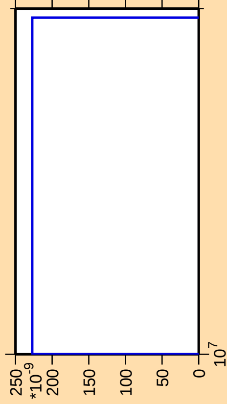
\Delta\sigma/\sigma vs. E for ^{51}\text{Mn}(\text{mt } 34)
