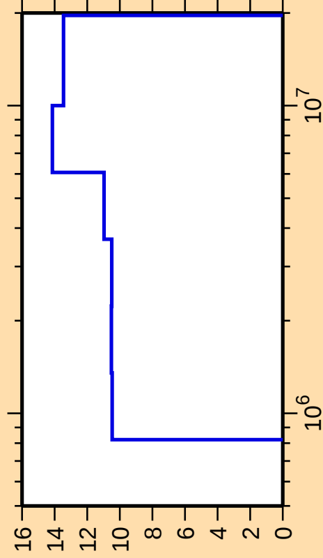
\Delta\sigma/\sigma vs. E for ^{51}\text{Mn}(n,n_2)
