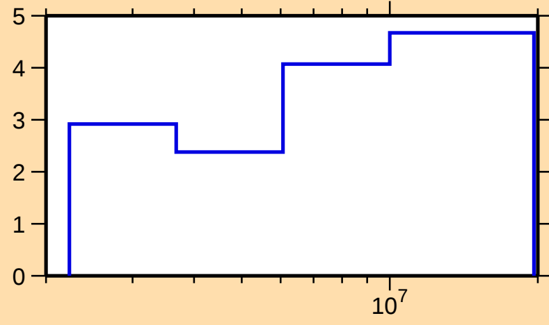
\Delta\sigma/\sigma vs. E for ^{51}\text{Mn}(n,\text{el.})
