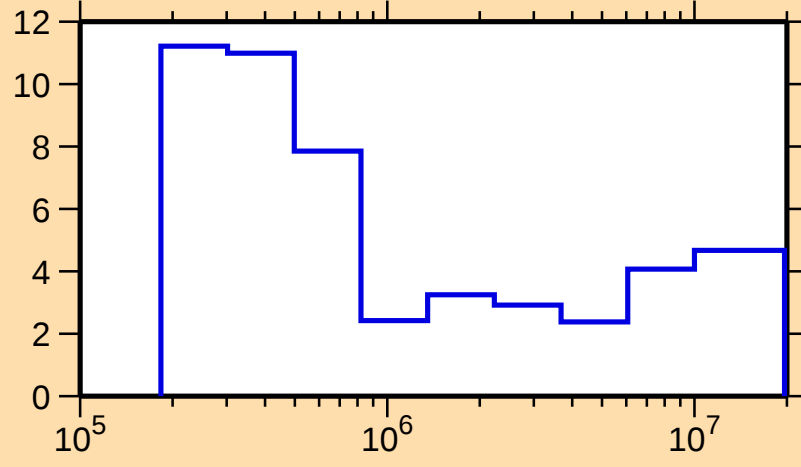
\Delta\sigma/\sigma vs. E for ^{51}\text{Mn}(n,\text{el.})
