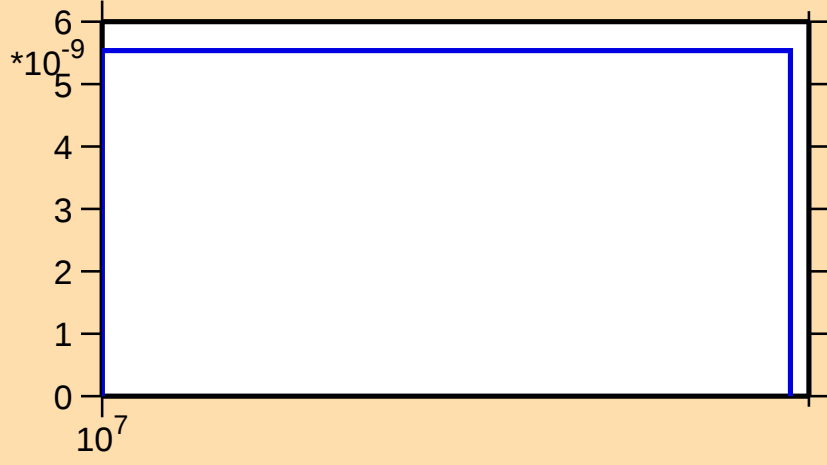
\sigma vs. E for ^{51}\text{Mn}(n,\text{nd})
