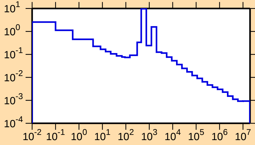
\sigma vs. E for ^{51}\text{Mn}(n,\gamma)
