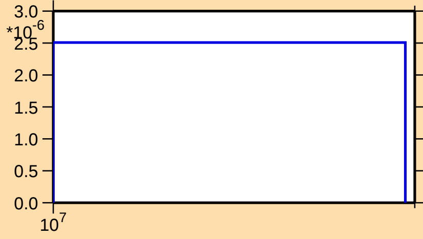
\sigma vs. E for ^{51}\text{Mn}(n,\text{pd})
