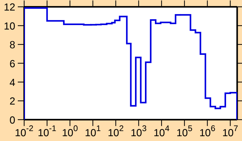
\Delta\sigma/\sigma vs. E for ^{51}\text{Mn}(n,\text{tot.})
