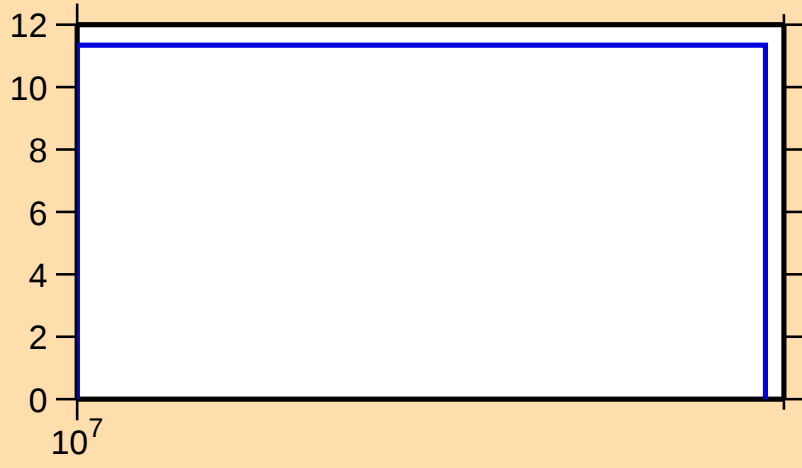
\Delta\sigma/\sigma vs. E for ^{51}\text{Mn}(n,\text{inel.})
