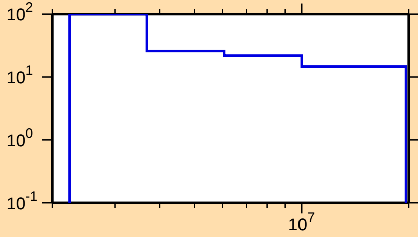
\Delta\sigma/\sigma vs. E for ^{51}\text{Mn}(n,n\text{cont.})
