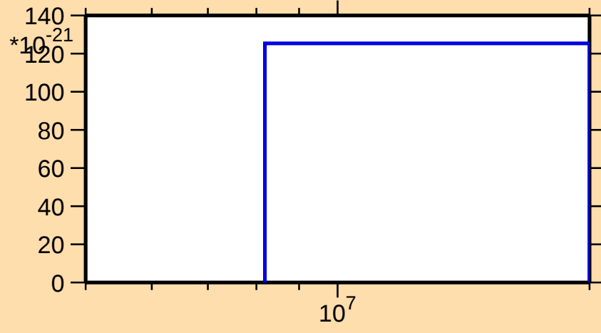
\sigma vs. E for ^{51}\text{Mn}(\text{mt } 34)
