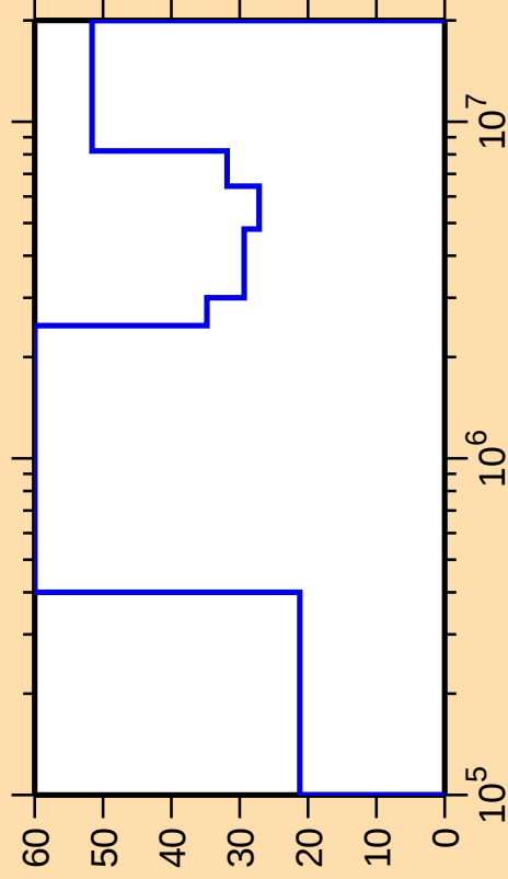
\Delta\sigma/\sigma vs. E for ^{51}\text{Mn}(n,\alpha)
