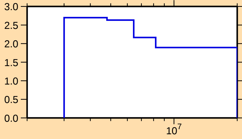
\Delta\sigma/\sigma vs. E for ^{51}\text{Mn}(n,n\text{onrel.})
