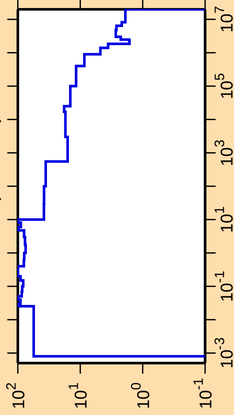
\Delta\sigma/\sigma vs. E for ^{51}\text{Mn}(n,\text{nonel.})
