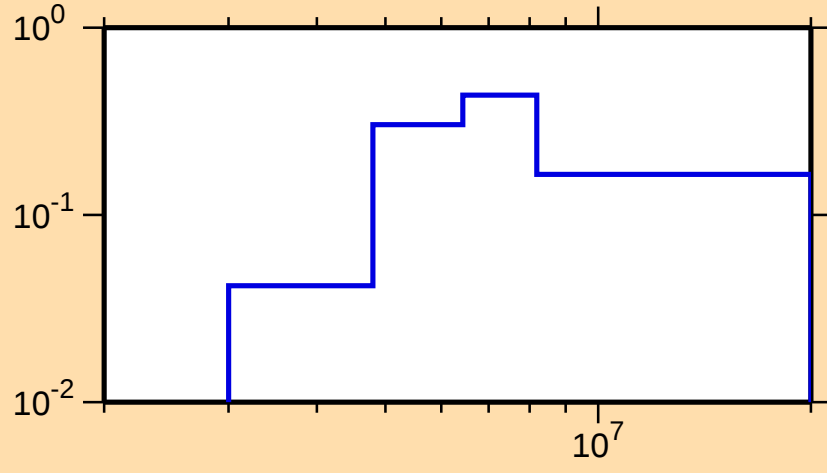
\sigma vs. E for ^{51}\text{Mn}(n,n\text{cont.})
