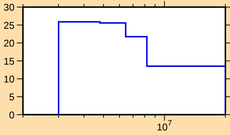
\Delta\sigma/\sigma vs. E for ^{51}\text{Mn}(n,n\text{cont.})
