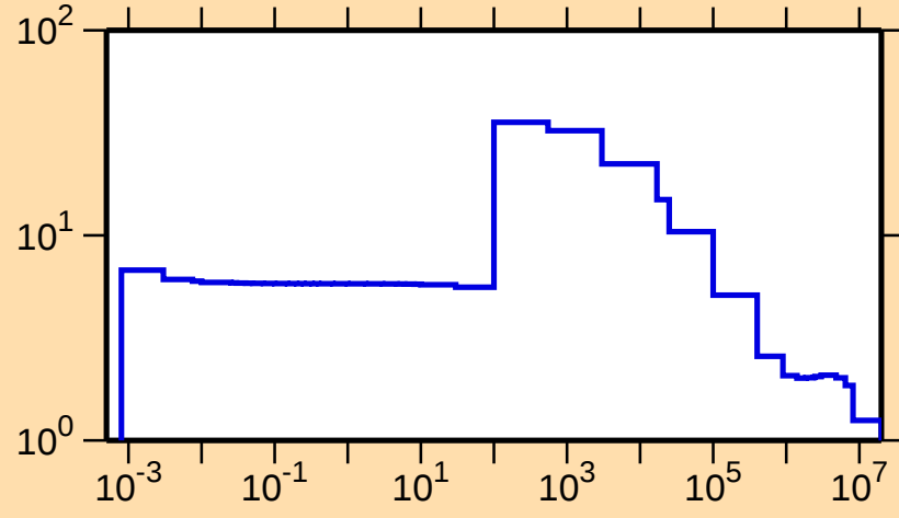
\sigma vs. E for ^{51}\text{Mn}(n,\text{el.})
