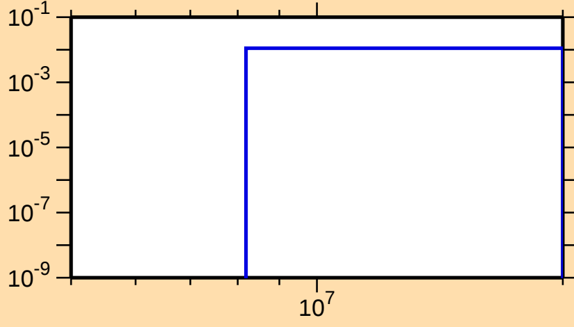
\sigma vs. E for ^{51}\text{Mn}(n,p\alpha)
