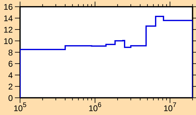
\Delta\sigma/\sigma vs. E for ^{51}\text{Mn}(n,n_1)
