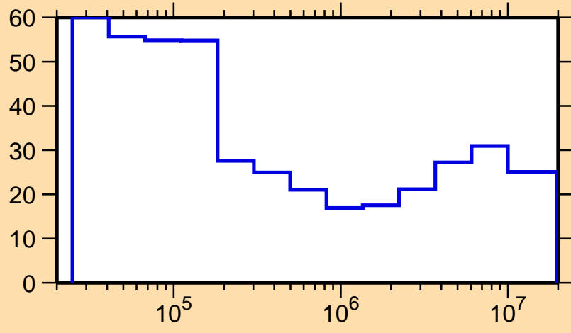
\Delta\sigma/\sigma vs. E for ^{87}\text{Mo}(n,n_1)
