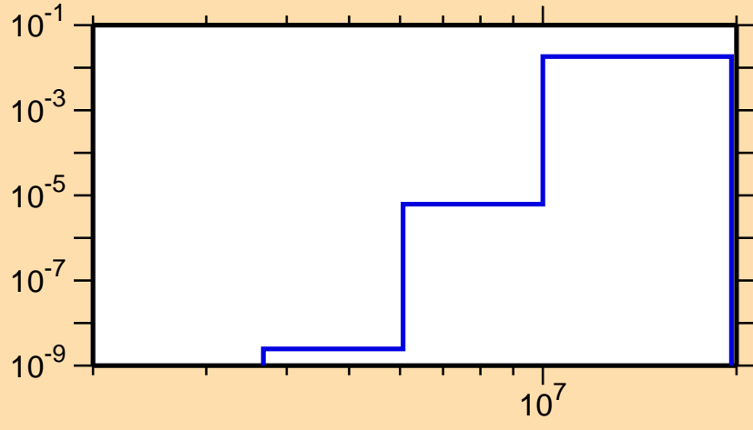
\sigma vs. E for ^{87}\text{Mo}(n,d)
