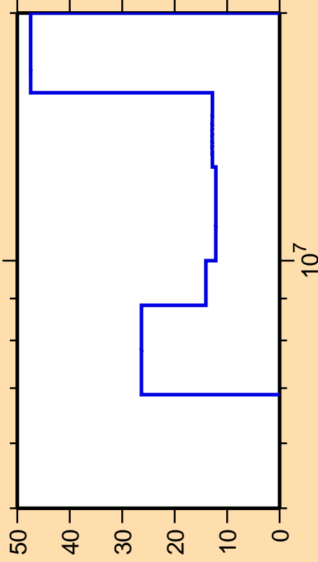
\Delta\sigma/\sigma vs. E for ^{104}\text{Mo}(n,2n)
