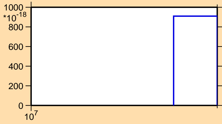
\sigma vs. E for ^{104}\text{Mo}(n,2np)
