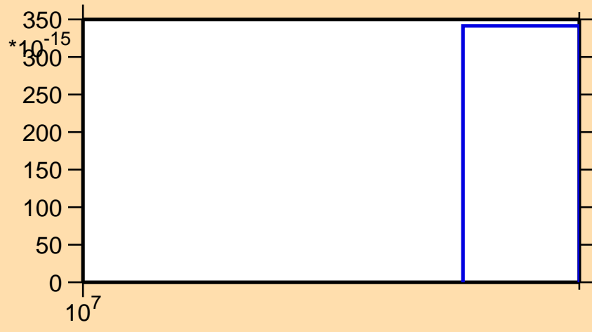
\sigma vs. E for ^{107}\text{Mo}(n,2np)
