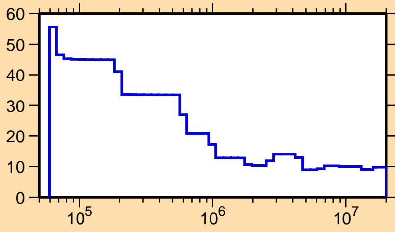
\Delta\sigma/\sigma vs. E for ^{107}\text{Mo}(n,\text{nonel.})
