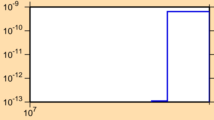
\sigma vs. E for ^{107}\text{Mo}(n,2n\alpha)
