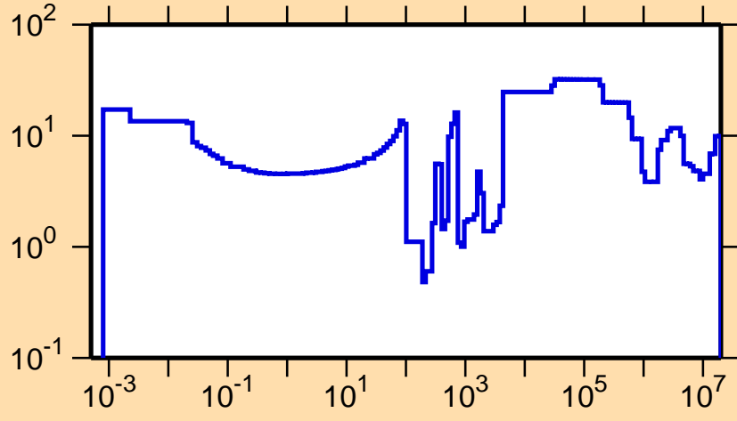
\Delta\sigma/\sigma vs. E for ^{107}\text{Mo}(n,\text{tot.})
