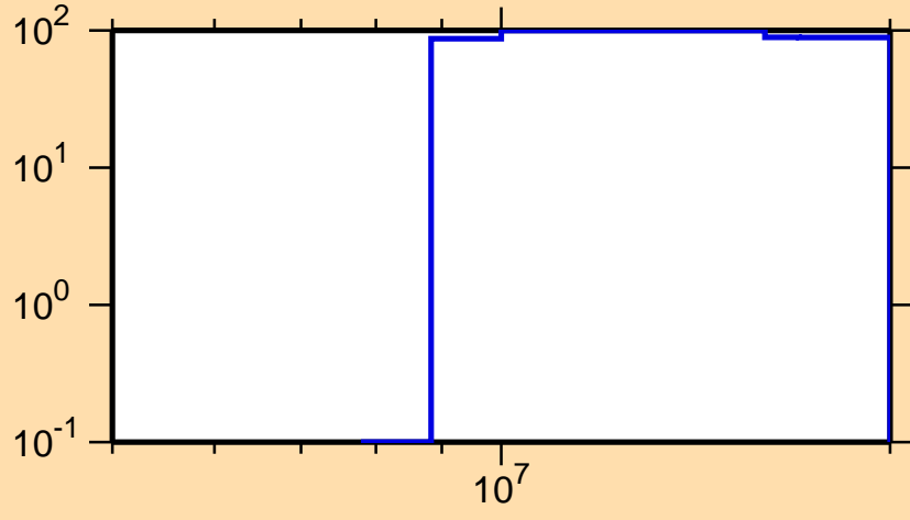
\Delta\sigma/\sigma vs. E for ^{107}\text{Mo}(n,p)
