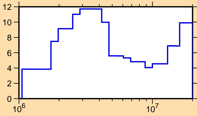
\Delta\sigma/\sigma vs. E for ^{107}\text{Mo}(n,\text{tot.})
