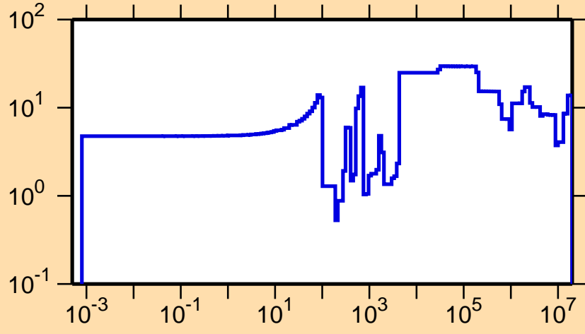
\Delta\sigma/\sigma vs. E for ^{107}\text{Mo}(n,\text{el.})
