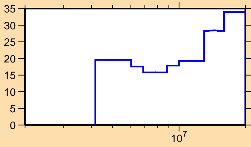
\Delta\sigma/\sigma vs. E for ^{107}\text{Mo}(n,2n)
