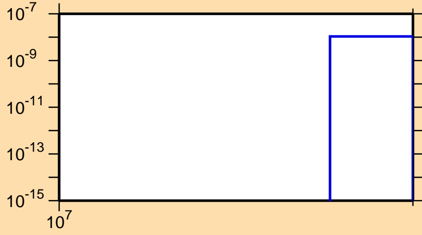
\sigma vs. E for ^{107}\text{Mo}(n,\text{nd})
