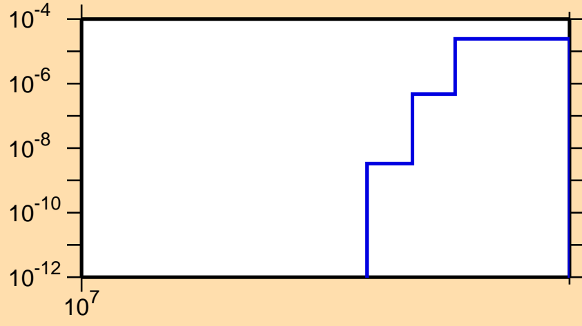
\sigma vs. E for ^{107}\text{Mo}(n,np)
