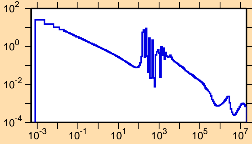
\sigma vs. E for ^{107}\text{Mo}(n,\gamma)
