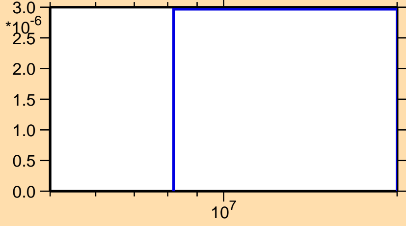
\sigma vs. E for ^{107}\text{Mo}(n,d)
