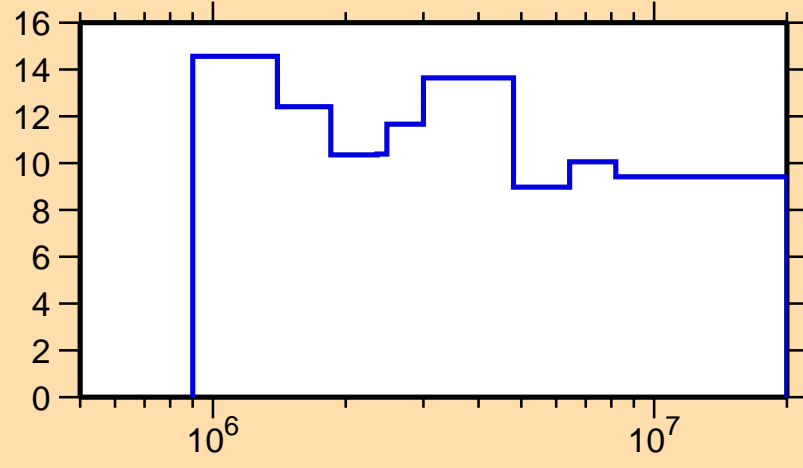
\Delta\sigma/\sigma vs. E for ^{107}\text{Mo}(n,n\text{onel.})
