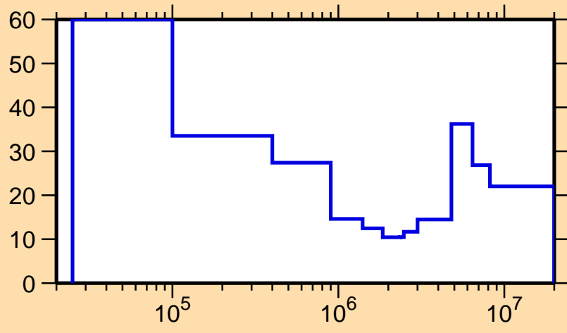
\Delta\sigma/\sigma vs. E for ^{107}\text{Mo}(n,\text{inel.})
