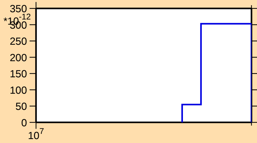
\sigma vs. E for ^{277}\text{He3}
