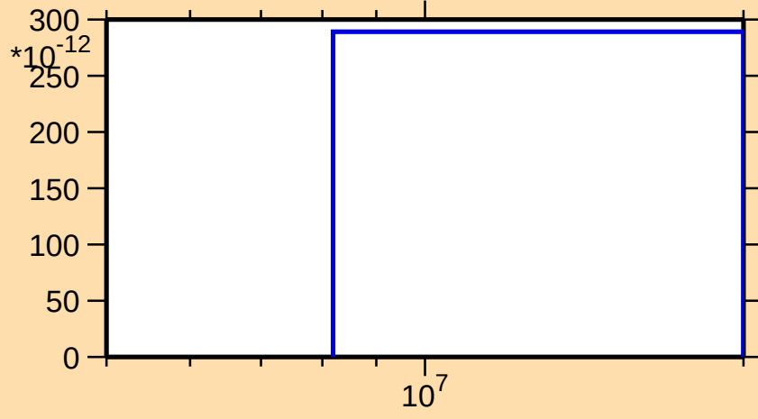
\sigma vs. E for ^{277}\alpha )
