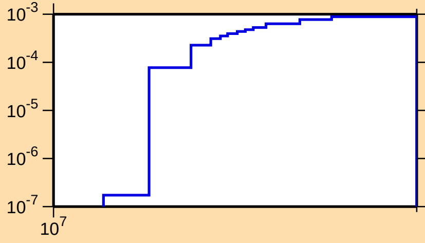
\sigma vs. E for ^{84}\text{Nb}(n,2n)
