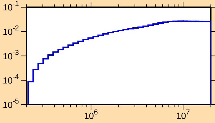
\sigma vs. E for ^{84}\text{Nb}(n,n_4)
