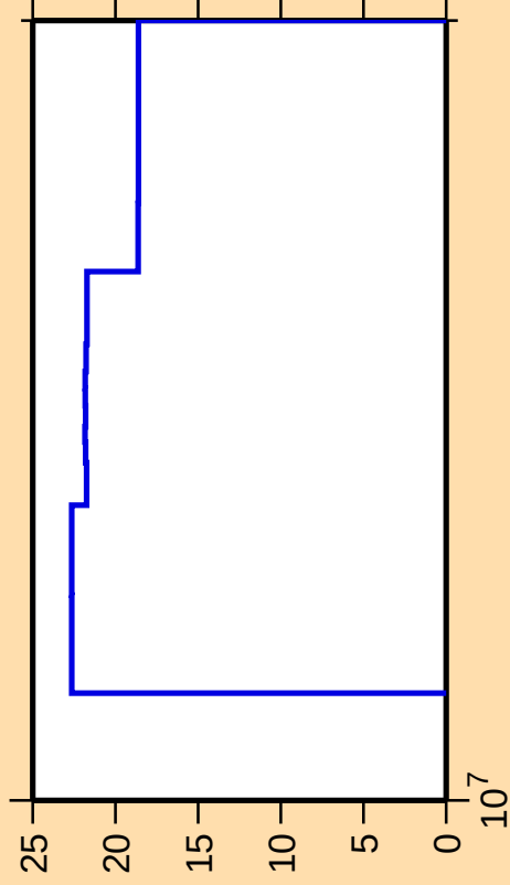
\Delta\sigma/\sigma vs. E for ^{84}\text{Nb}(n,n_{\text{cont}})
