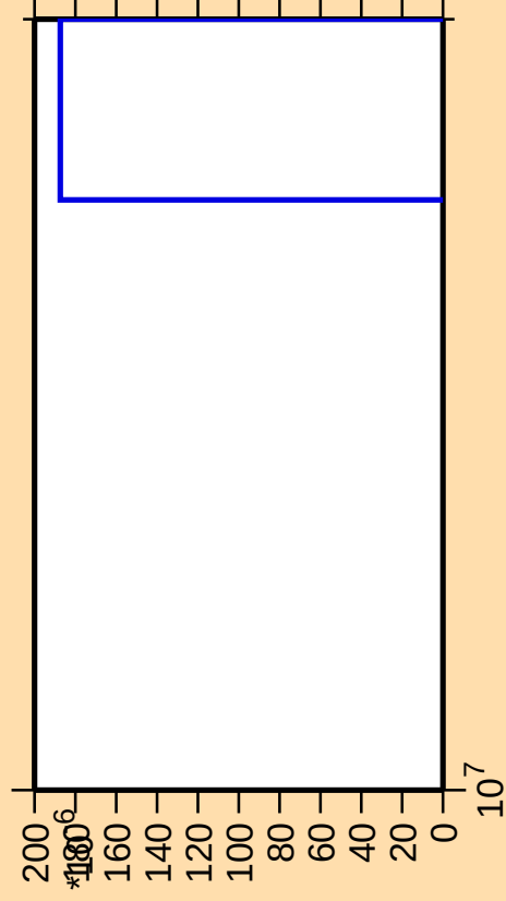
\Delta\sigma/\sigma vs. E for ^{84}\text{Nb}(n,nt)
