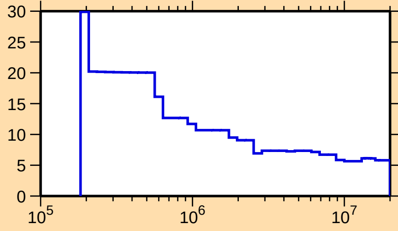
\Delta\sigma/\sigma vs. E for ^{84}\text{Nb}(n,n\text{onel.})
