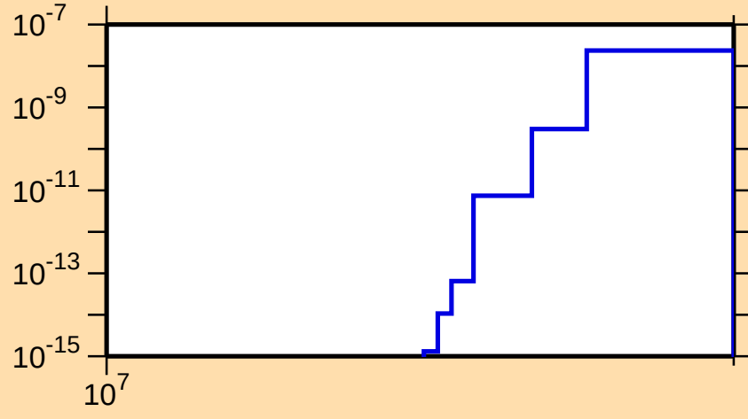
\sigma vs. E for ^{84}\text{Nb}(\text{mt } 34)
