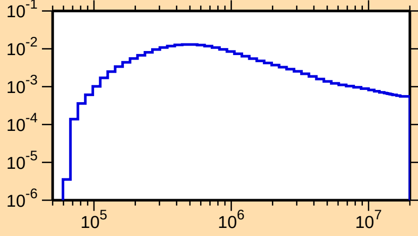
\sigma vs. E for ^{84}\text{Nb}(n,n_2)
