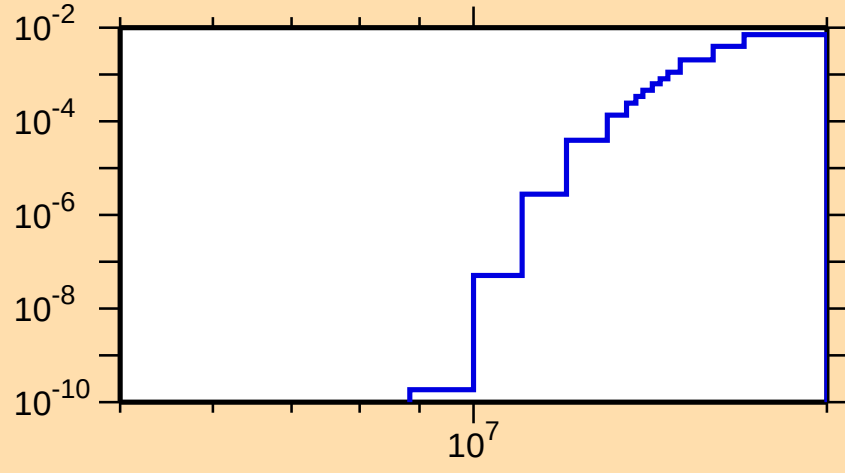
\sigma vs. E for ^{84}\text{Nb}(n,\text{pd})
