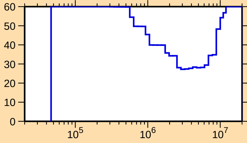
\Delta\sigma/\sigma vs. E for ^{84}\text{Nb}(n,n_1)
