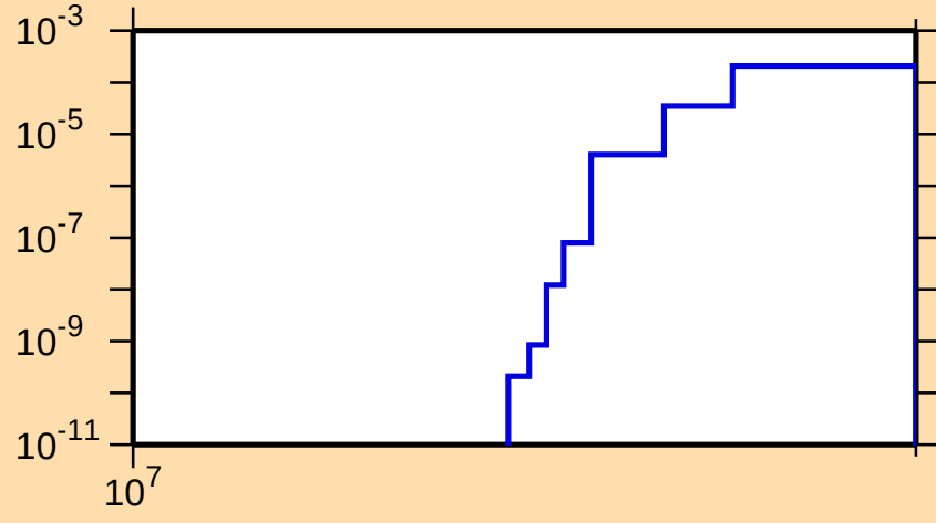
\sigma vs. E for ^{84}\text{Nb}(n,2np)
