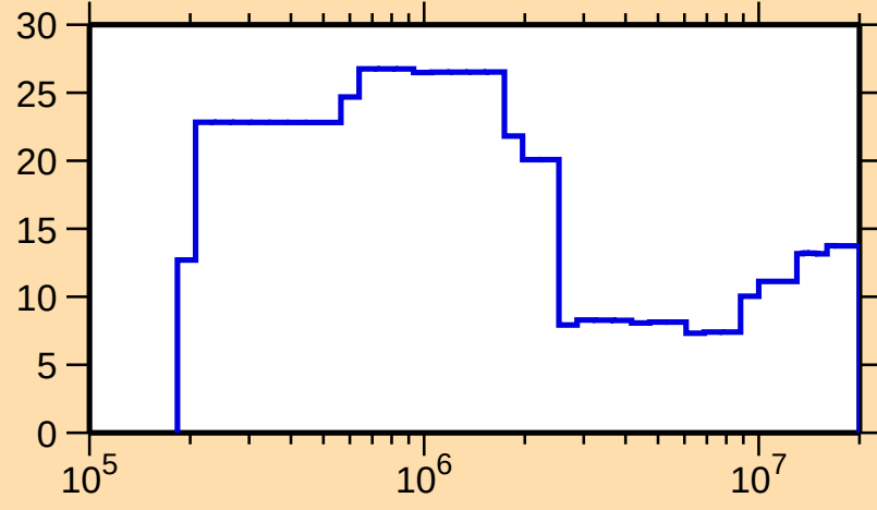
\Delta\sigma/\sigma vs. E for ^{84}\text{Nb}(n,\text{el.})
