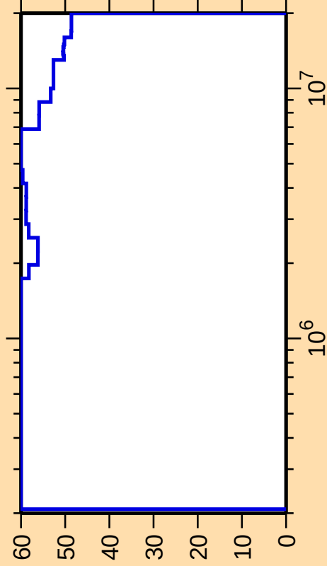
\Delta\sigma/\sigma vs. E for ^{84}\text{Nb}(n,n_4)
