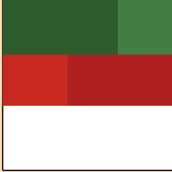
\Delta\sigma/\sigma vs. E for ^{84}\text{Nb}(n,\text{nonel.})
