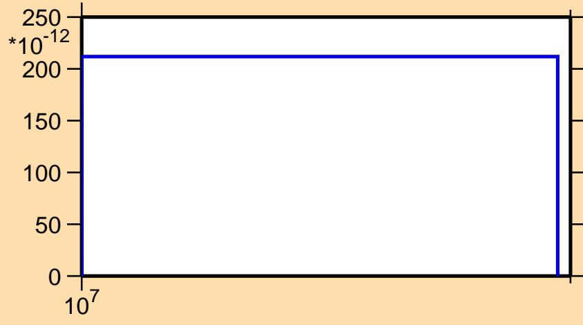
\sigma vs. E for ^{84}\text{Nb} (mt 34)
