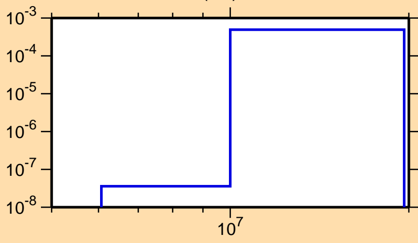
\sigma vs. E for ^{84}\text{Nb}(n,t)
