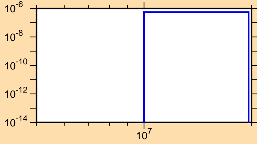
\sigma vs. E for ^{84}\text{Nb} (mt 45)
