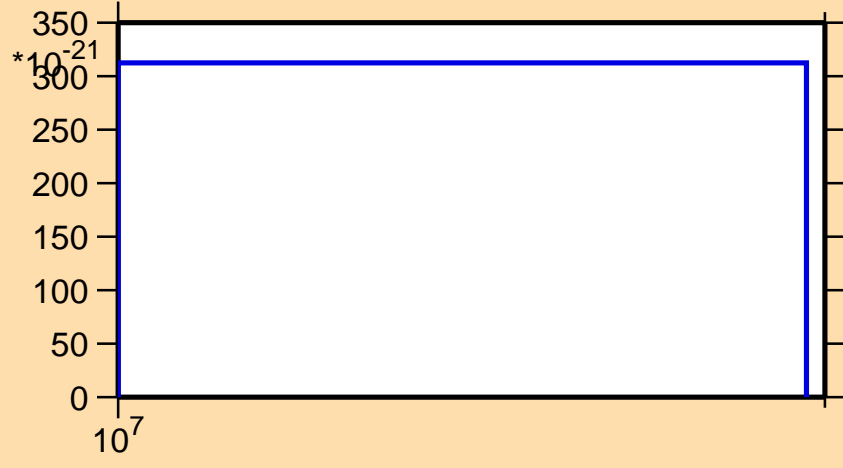
\sigma vs. E for ^{84}\text{Nb}(n,nt)
