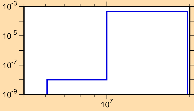
\sigma vs. E for ^{84}\text{Nb}(n,n\alpha)
