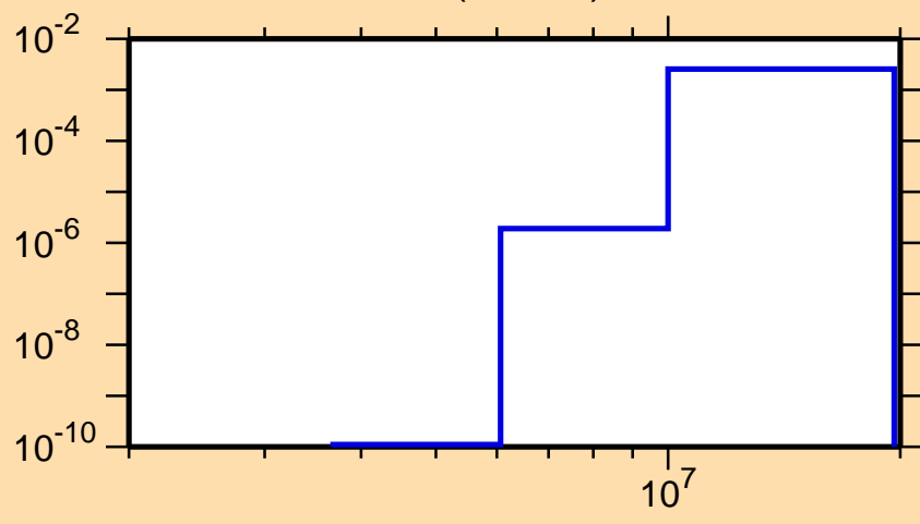
\sigma vs. E for ^{84}\text{Nb}(n,\text{He3})
