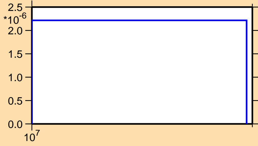
\sigma vs. E for ^{84}\text{Nb}(n,\text{pt})
