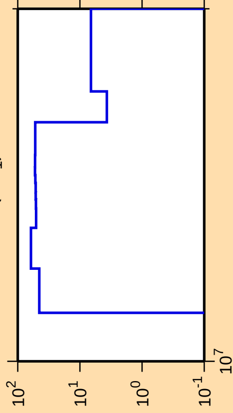
\Delta\sigma/\sigma vs. E for ^{86}\text{Nb}(n,n_1)
