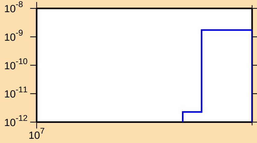
\sigma vs. E for ^{86}\text{Nb}(\text{mt } 34)
