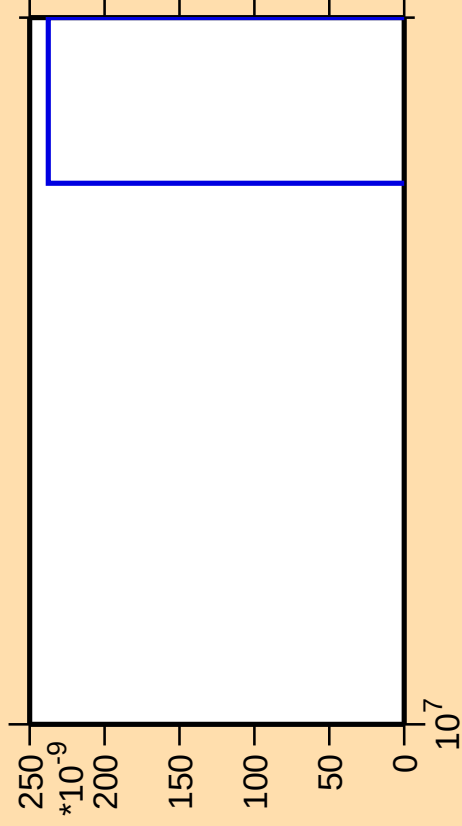
\Delta\sigma/\sigma vs. E for ^{86}\text{Nb}(n,nt)
