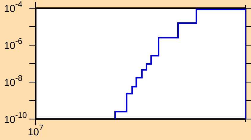
\sigma vs. E for ^{86}\text{Nb}(n,\text{nd})
