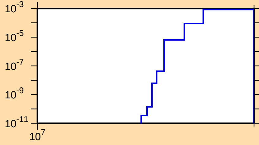
\sigma vs. E for ^{86}\text{Nb}(n,2np)
