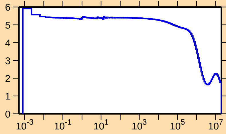
\sigma vs. E for ^{86}\text{Nb}(n,\text{el.})
