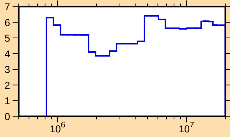
\Delta\sigma/\sigma vs. E for ^{86}\text{Nb}(n,n\text{nonel.})
