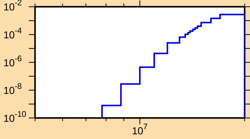
\sigma vs. E for ^{86}\text{Nb}(n,\text{He3})
