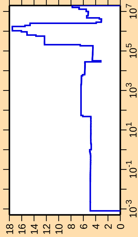
\Delta\sigma/\sigma vs. E for ^{86}\text{Nb}(n,\text{el.})
