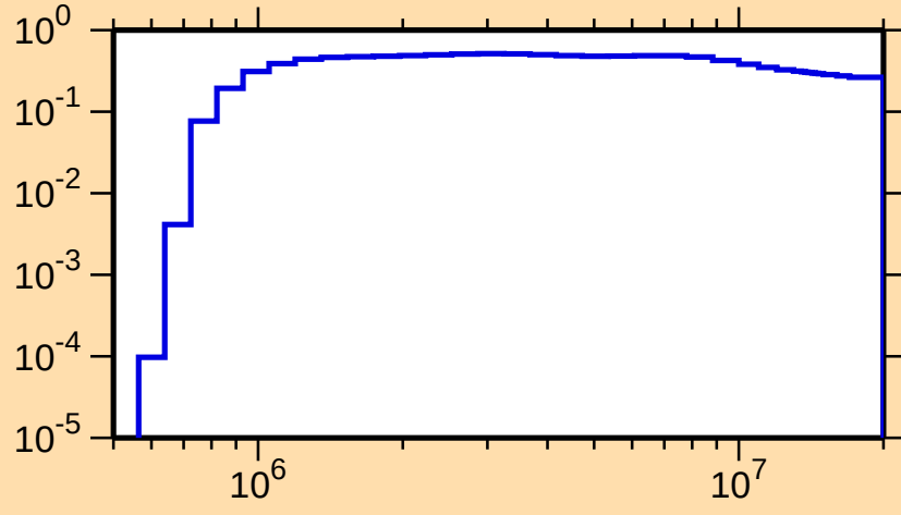
\sigma vs. E for ^{86}\text{Nb}(n,\text{inel.})
