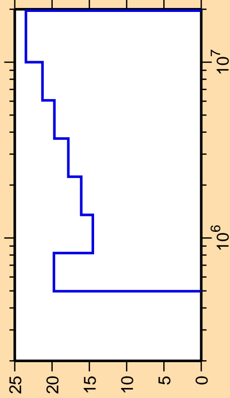
\Delta\sigma/\sigma vs. E for ^{86}\text{Nb}(n,n_4)
