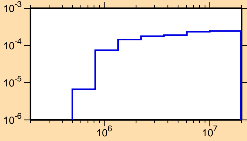
\sigma vs. E for ^{86}\text{Nb}(n,n_4)
