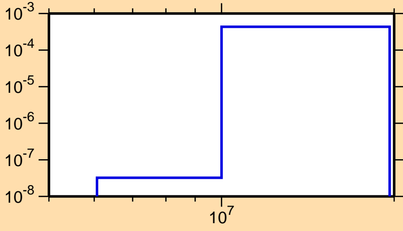
\sigma vs. E for ^{86}\text{Nb}(n,t)
