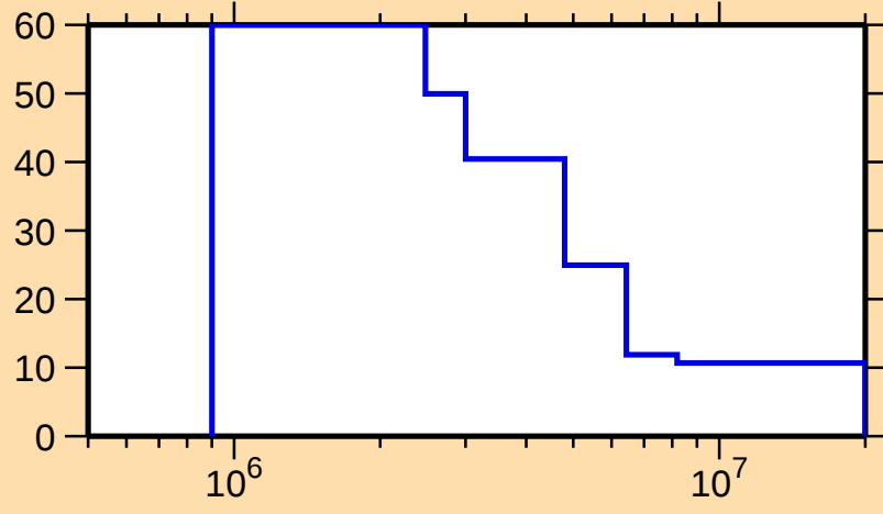
\Delta\sigma/\sigma vs. E for ^{86}\text{Nb}(n,n\text{cont.})
