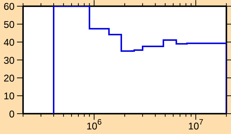
\Delta\sigma/\sigma vs. E for ^{86}\text{Nb}(n,n_1)
