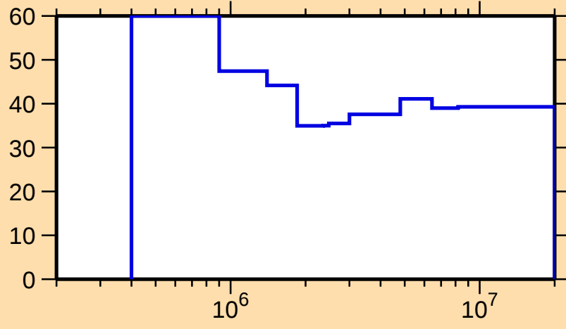
\Delta\sigma/\sigma vs. E for ^{86}\text{Nb}(n,n_1)
