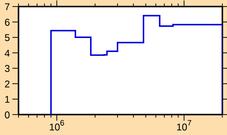
\Delta\sigma/\sigma vs. E for ^{86}\text{Nb}(n,n\text{onel.})
