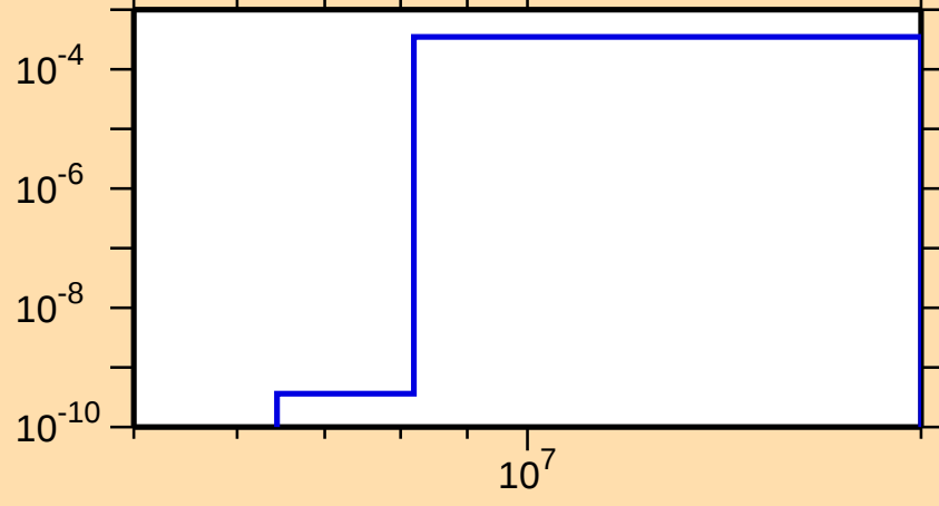
\sigma vs. E for ^{86}\text{Nb}(n,t)
