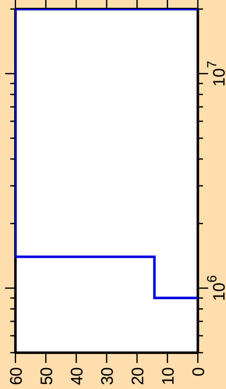
\Delta\sigma/\sigma vs. E for ^{86}\text{Nb}(n,p\alpha)
