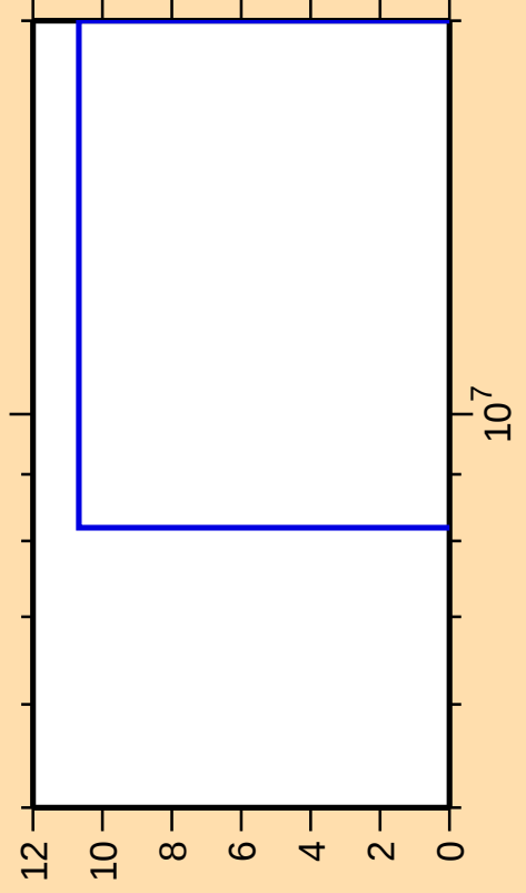
\Delta\sigma/\sigma vs. E for ^{86}\text{Nb}(n,n\text{cont.})
