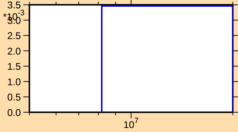
\sigma vs. E for ^{86}\text{Nb}(n,2n)
