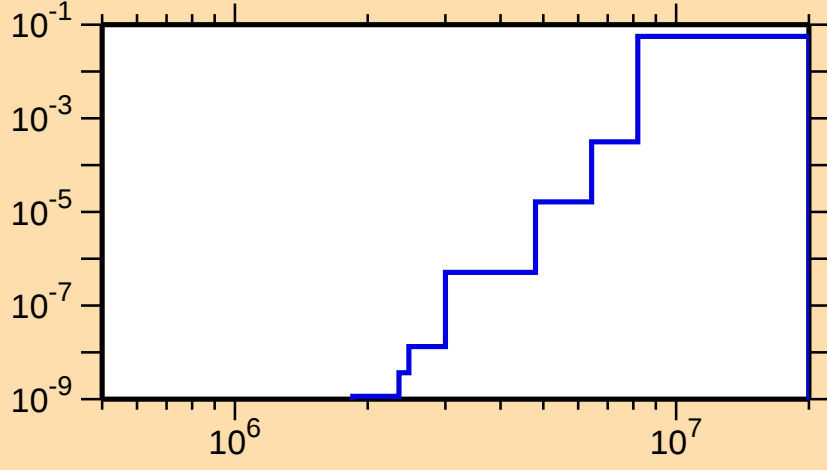
\sigma vs. E for ^{86}\text{Nb}(n,p\alpha)
