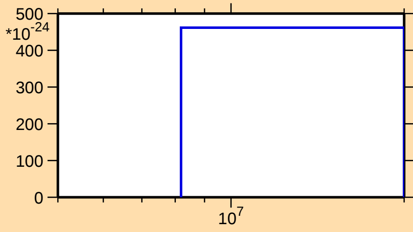
\sigma vs. E for ^{86}\text{Nb}(n,nt)
