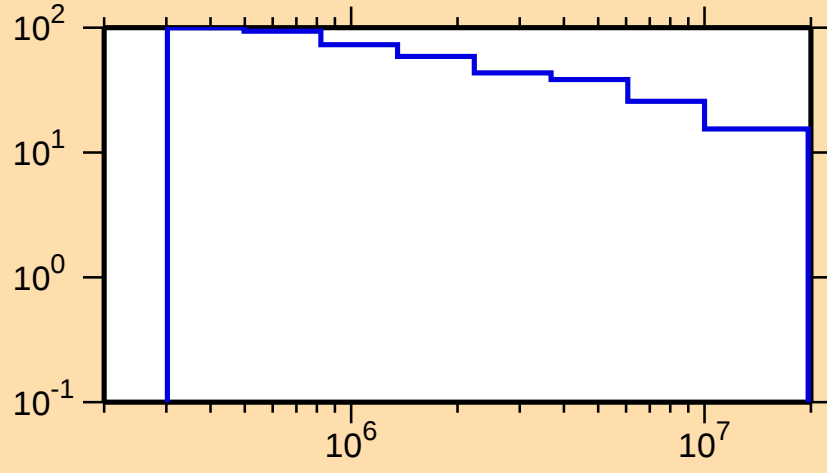
\Delta\sigma/\sigma vs. E for ^{86}\text{Nb}(n,n\text{cont.})
