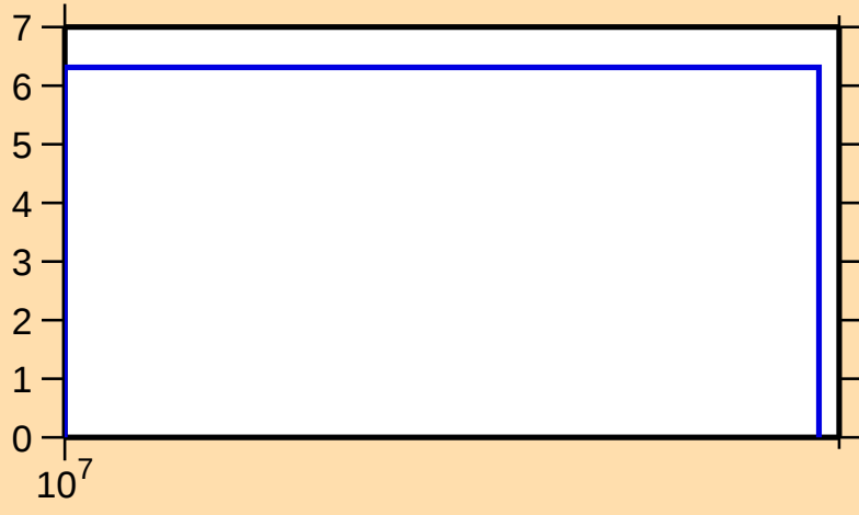
\Delta\sigma/\sigma vs. E for ^{86}\text{Nb}(n,\text{el.})
