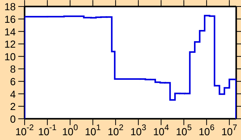
\Delta\sigma/\sigma vs. E for ^{86}\text{Nb}(n,\text{el.})
