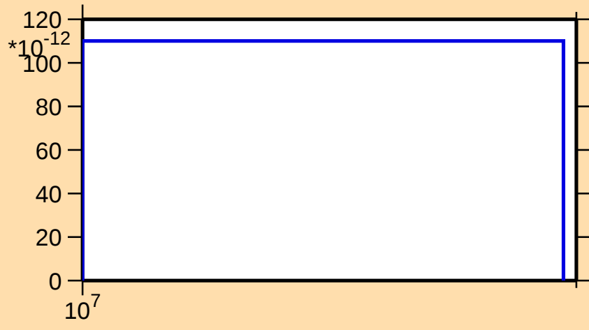
\sigma vs. E for ^{86}\text{Nb}(\text{mt } 34)
