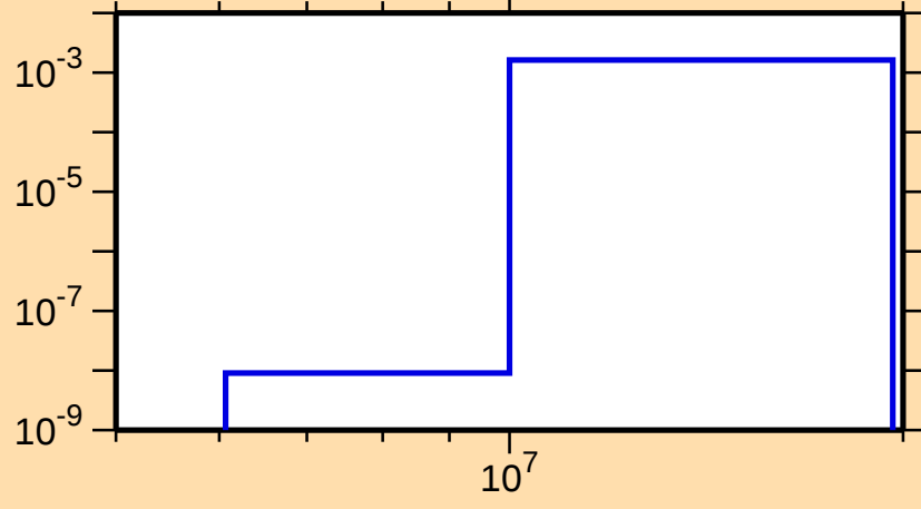
\sigma vs. E for ^{86}\text{Nb}(n,n\alpha)
