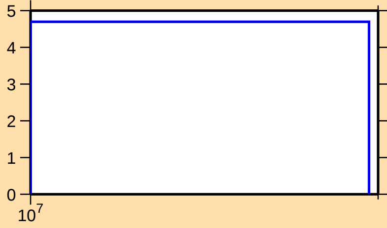
\Delta\sigma/\sigma vs. E for ^{86}\text{Nb}(n,\text{tot.})
