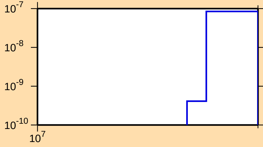
\sigma vs. E for ^{88}\text{Nb}(\text{mt } 45)
