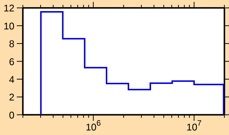
\Delta\sigma/\sigma vs. E for ^{88}\text{Nb}(n,n\text{nonel.})
