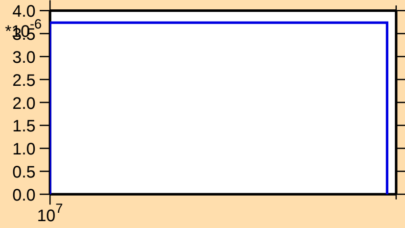
\sigma vs. E for ^{88}\text{Nb}(n,\text{nd})
