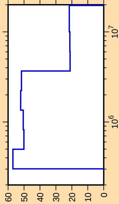
\Delta\sigma/\sigma vs. E for ^{88}\text{Nb}(n,\text{ncont.})
