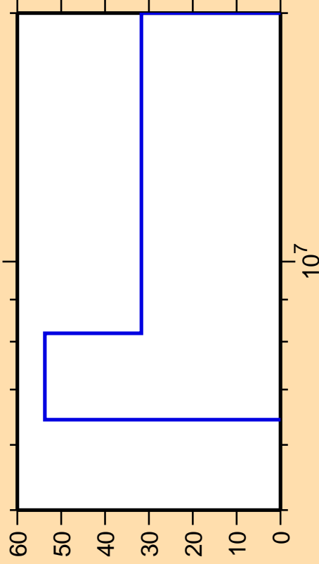
\Delta\sigma/\sigma vs. E for ^{92}\text{Nb}(n,p\alpha)
