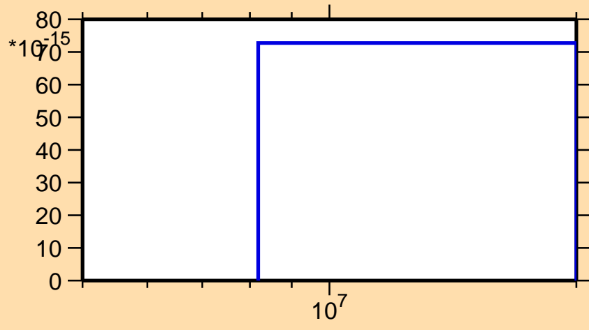
\sigma vs. E for ^{92}\text{Nb}(\text{mt } 34)
