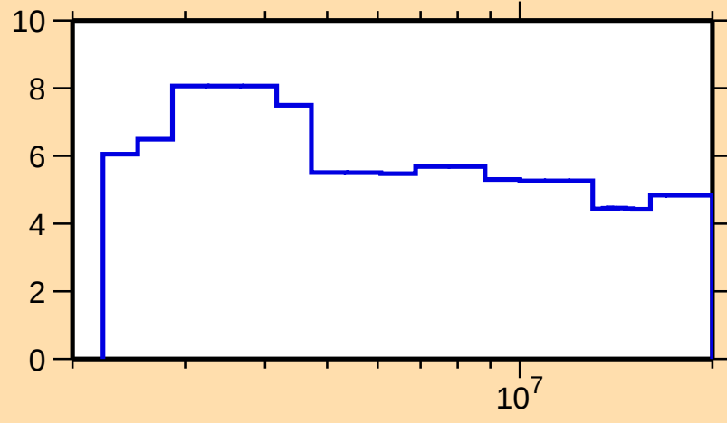
\Delta\sigma/\sigma vs. E for ^{99}\text{Nb}(n,n\text{nonel.})
