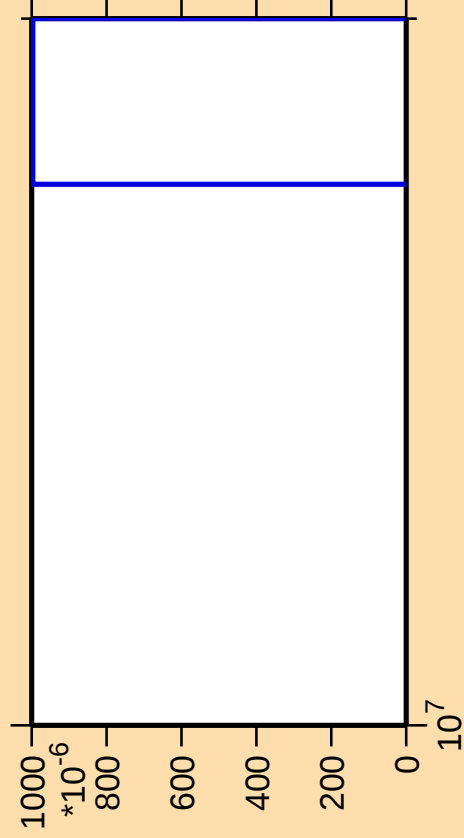
\Delta\sigma/\sigma vs. E for ^{99}\text{Nb}(\text{mt } 11)
