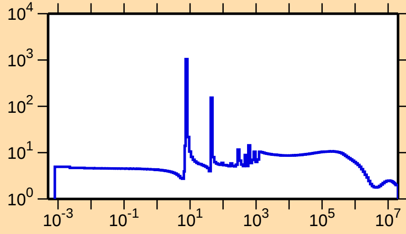
\sigma vs. E for ^{99}\text{Nb}(n,\text{el.})
