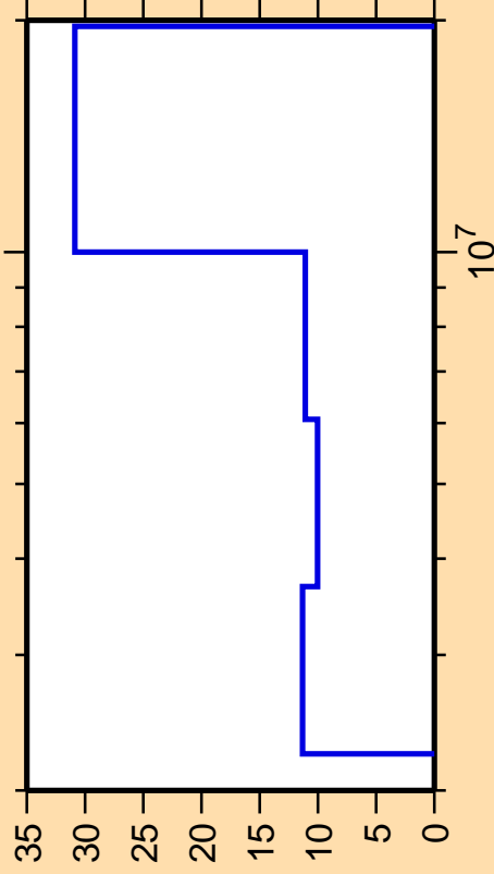
\Delta\sigma/\sigma vs. E for ^{99}\text{Nb}(n,n\text{cont.})
