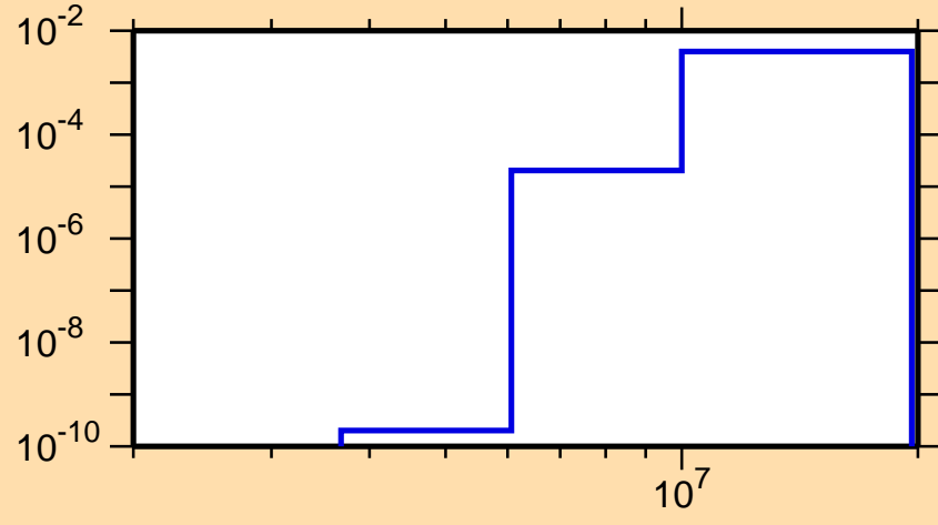
\sigma vs. E for ^{99}\text{Nb}(n,p)
