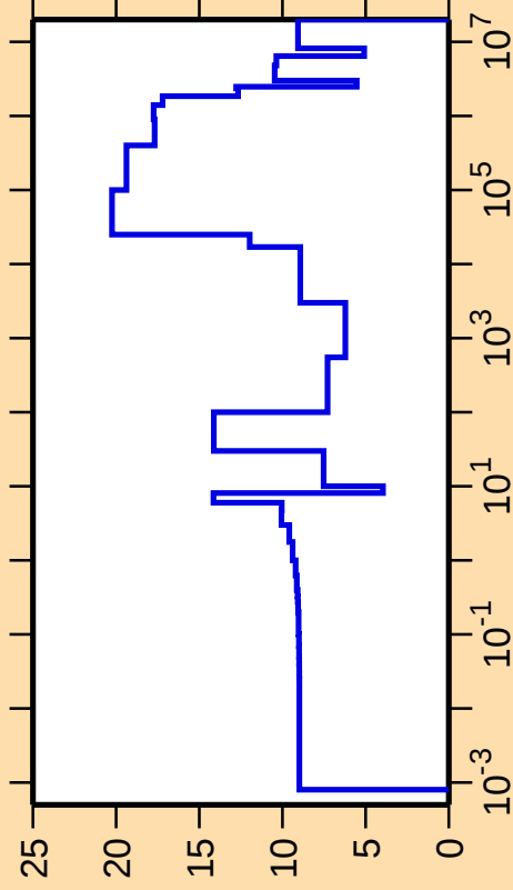
\Delta\sigma/\sigma vs. E for ^{99}\text{Nb}(n,\text{el.})
