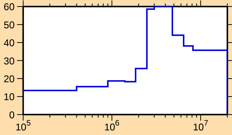
\Delta\sigma/\sigma vs. E for ^{99}\text{Nb}(n,n_1)
