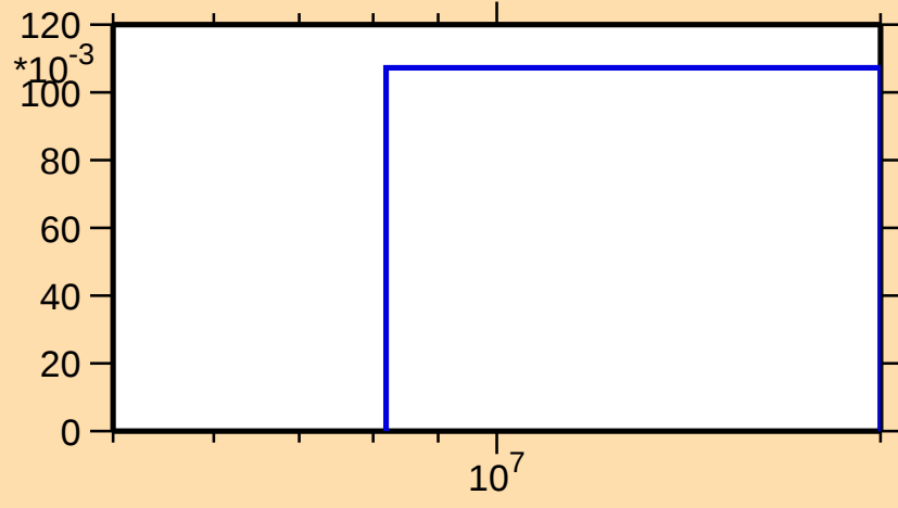
\sigma vs. E for ^{99}\text{Nb}(n,3n)
