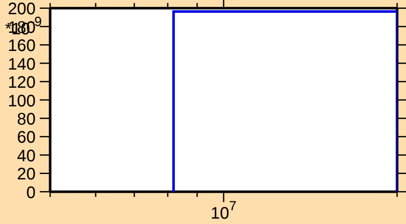
\sigma vs. E for ^{99}\text{Nb}(n,\text{nd})
