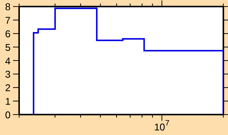
\Delta\sigma/\sigma vs. E for ^{99}\text{Nb}(n,n\text{nonel.})
