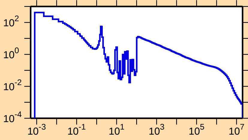
\sigma vs. E for ^{128}\text{Nd}(n,\gamma)
