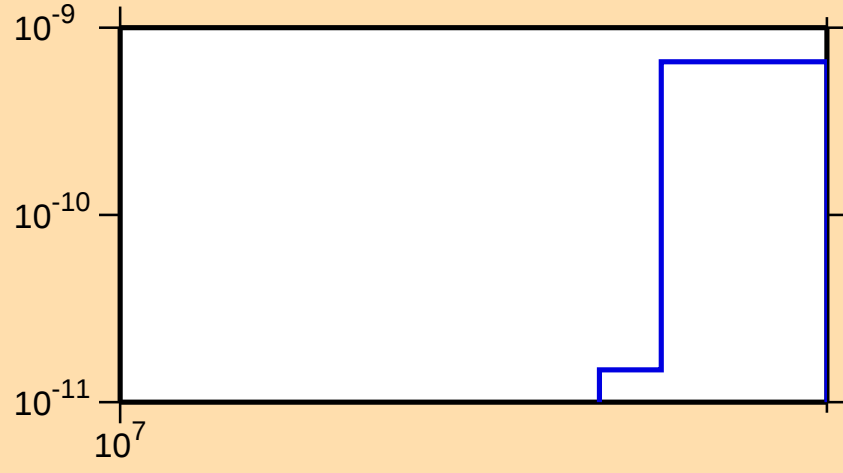
\sigma vs. E for ^{128}\text{Nd} (mt 34)
