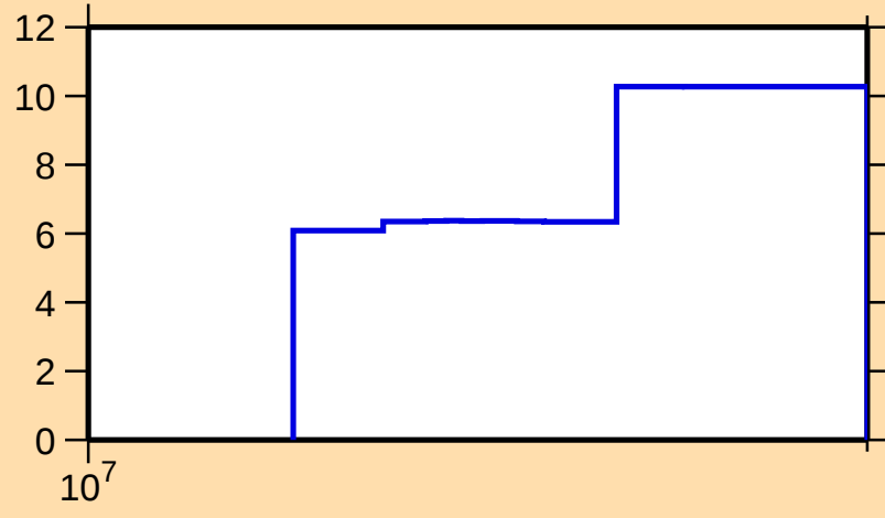
\Delta\sigma/\sigma vs. E for ^{128}\text{Nd}(n,\text{el.})
