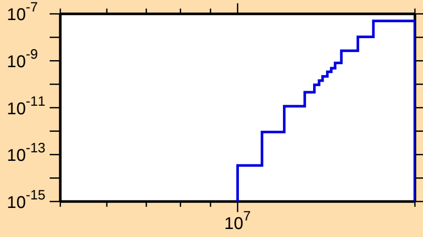
\sigma vs. E for ^{128}\text{Nd}(\text{mt117})
