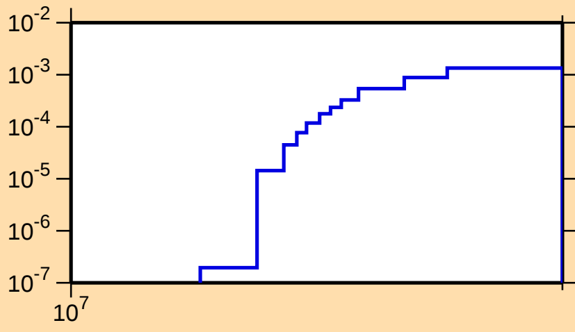
\sigma vs. E for ^{128}\text{Nd}(n,2n)
