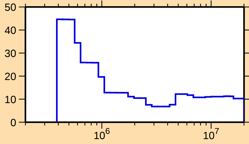
\Delta\sigma/\sigma vs. E for ^{128}\text{Nd}(n,n\text{onel.})
