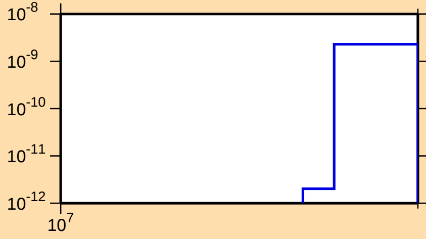
\sigma vs. E for ^{128}\text{Nd}(n,\text{nd})
