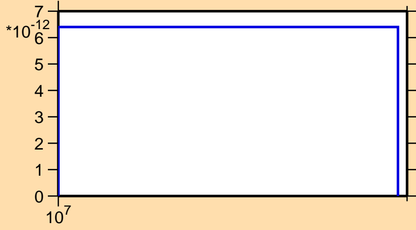
\sigma vs. E for ^{128}\text{Nd} (mt 34)
