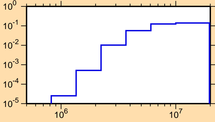
\sigma vs. E for ^{128}\text{Nd}(n,n\text{cont.})
