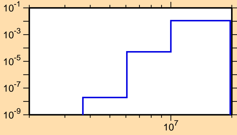
\sigma vs. E for ^{128}\text{Nd}(n,d)
