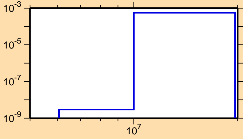
\sigma vs. E for ^{128}\text{Nd}(n,\text{pd})
