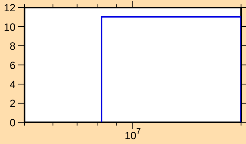
\Delta\sigma/\sigma vs. E for ^{128}\text{Nd}(n,\text{nonel.})
