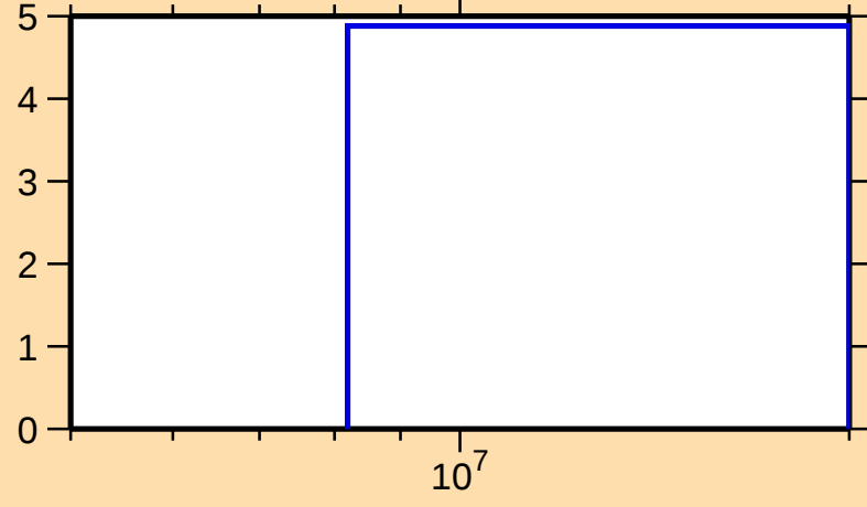
\Delta\sigma/\sigma vs. E for ^{128}\text{Nd}(n,\text{el.})
