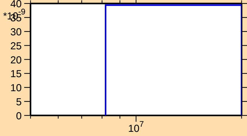
\sigma vs. E for ^{128}\text{Nd}(n,\text{pt})
