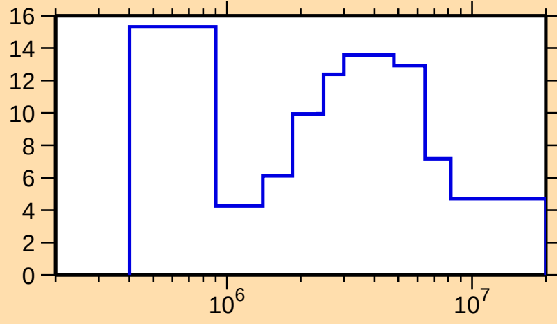
\Delta\sigma/\sigma vs. E for ^{128}\text{Nd}(n,\text{tot.})
