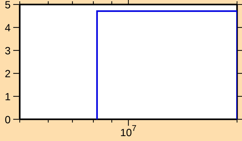
\Delta\sigma/\sigma vs. E for ^{128}\text{Nd}(n,\text{tot.})
