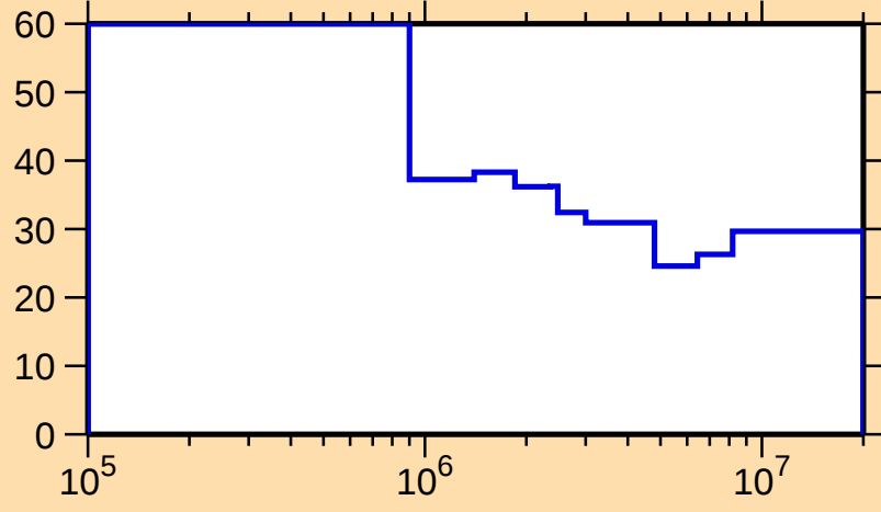
\Delta\sigma/\sigma vs. E for ^{128}\text{Nd}(n,n_1)
