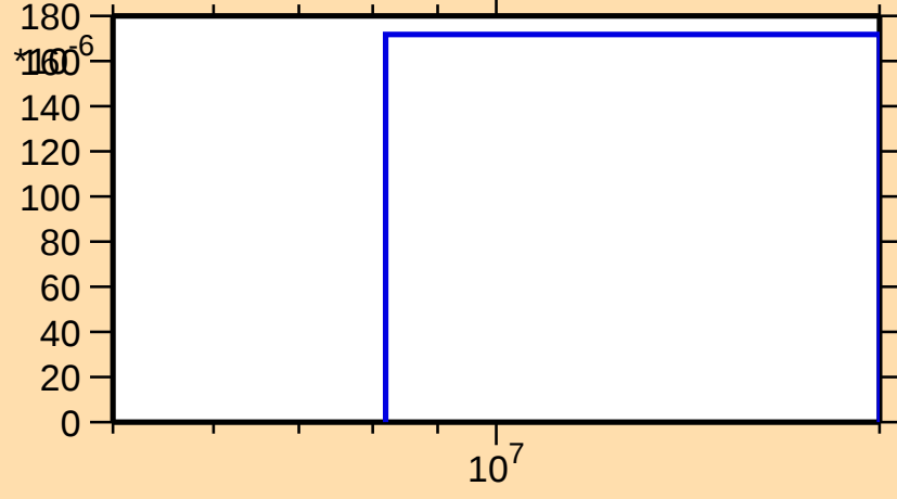
\sigma vs. E for ^{128}\text{Nd}(n,2n)
