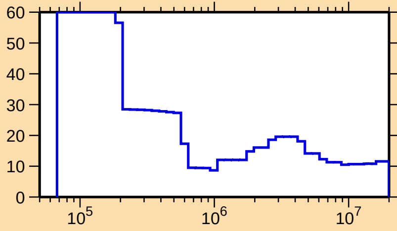
\Delta\sigma/\sigma vs. E for ^{156}\text{Nd}(n,\text{el.})
