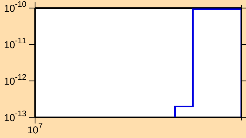
\sigma vs. E for ^{156}\text{Nd}(n,2n\alpha)
