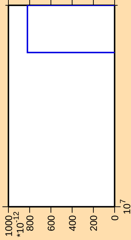
\Delta\sigma/\sigma vs. E for ^{156}\text{Nd} (mt 11)
